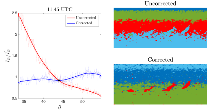
Figure 12: Illustration of the incidence angle correction applied to the UAVSAR scene acquired at 11:45 UTC. The left figure shows the smoothed mean VV-intensity profiles normalized to the mean of the span profile using the clean sea region before (red line) and after correction (blue line). The dotted lines are the unsmoothed mean intensity profiles. The black marker represents the reference level, i.e., mean of the span along the range direction. The right figures show the results of the segmentation with and without incidence angle correction. The colors represent the various output segments.
