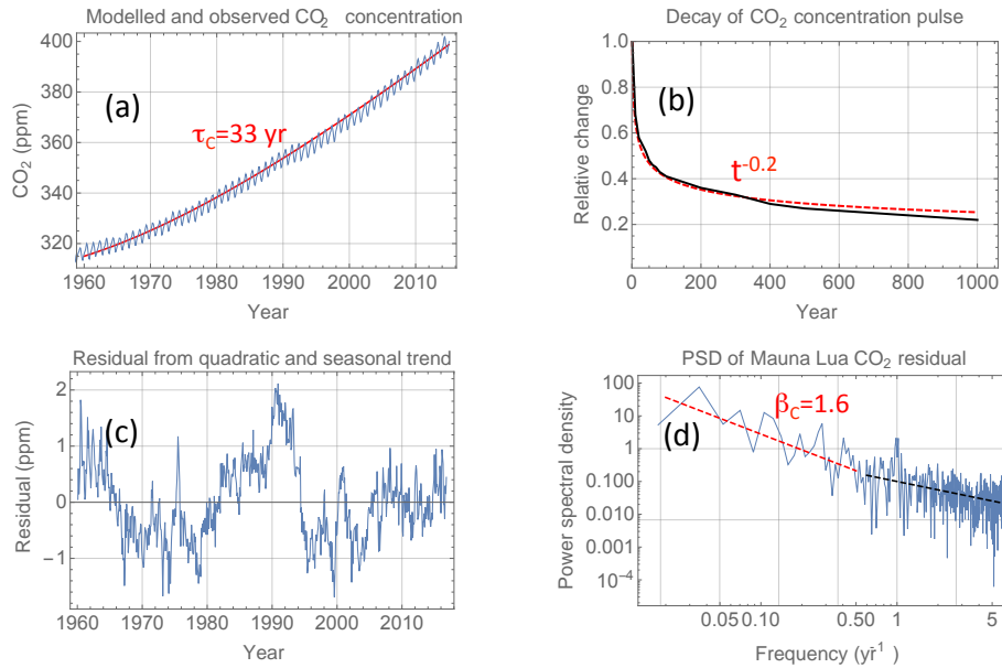
Figure 2. Panel (a): blue curve shows the atmospheric CO 2 concentration as measured by the Mauna Loa observatory. The red curve is the concentration computed from Eq. (5) with \tau_C = 33 years, \Delta C_{1960} = 74 Gt C (corresponding to an anomaly of 315 - 280 = 35 ppm), and C_0 = 594 Gt C (corresponding to 280 ppm). Panel (b): black curve is the multimodel mean CO 2 response to a pulse of emitted CO 2 as given in Joos et al. (2011). The red, dashed curve is a least-square fit of a function of the form \alpha_C t^{\beta_C/2-1} with the estimated \beta_C \approx 1.6 . Panel (c): the residual Mauna Loa signal after subtracting the quadratic polynomial and seasonal trends. Panel (d): the power spectral density of the residual in (c) estimated by the periodogram presented in a log–log plot. The black, dashed line has negative slope \beta_C = 0.85 , and the red, dashed line has \beta_C = 1.6 .
