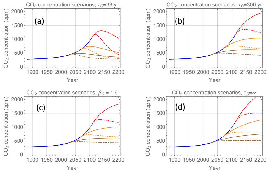
Figure 4. Projections of CO 2 concentration under the emission scenarios in Fig. 3 using the modelling explained in Sect. 2. The colours correspond to those in Fig. 3. Panel (a): \tau_C = 33 years; panel (b): \tau_C = 300 years; panel (c): \beta_C = 1.6 ; panel (d): \tau_C = \infty .
