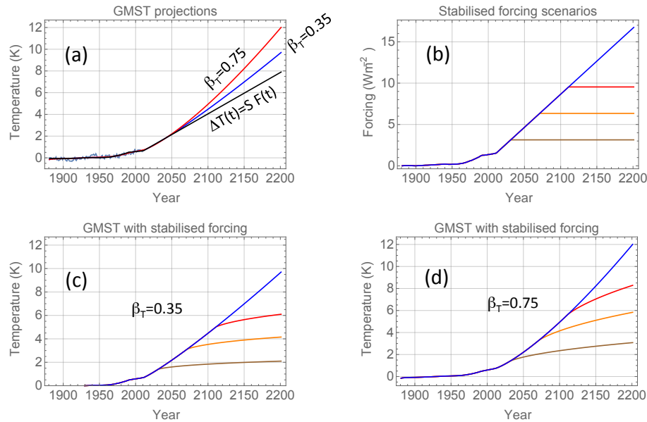
Figure 1. Panel (a): light blue curve is the instrumental GMST for 1880–2010 AD. Black curve is the instantaneous response to the linearly extrapolated forcing scenario shown in panel (b). Blue curve is the response according to the model Eq. (2) with \beta_T = 0.35 , and the red curve is the response with \beta_T = 0.75 . Panel (b): the straight sloping line is a linearly projected forcing to 2200 AD with the same mean growth rate as the RCP8.5 scenario in the period 2010–2100 AD. The horizontal line is the stabilisation of this forcing in 2030 AD, the horizontal orange line in 2070 AD, and the red horizontal line in 2110 AD. Panel (c): GMST responses to the forcing scenarios in (b) with \beta_T = 0.35 . Colours correspond to those in (b). Panel (d): same as in (c) but with \beta_T = 0.75 .
