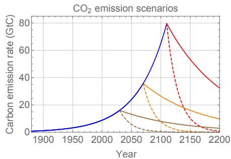
Figure 3. Blue curve is carbon emission rate R(t) scenario obtained by fitting the exponential S_0 \exp(gt) to the emission rate 4 \text{ Gt C yr}^{-1} in 1960 and 11 \text{ Gt C yr}^{-1} in 2010 AD. The solid, brown, orange, and red curves are the subsequent R(t) after initiation of a 1% reduction in the emission rate per year. The dashed curves are the corresponding rates with a 5% reduction per year.
