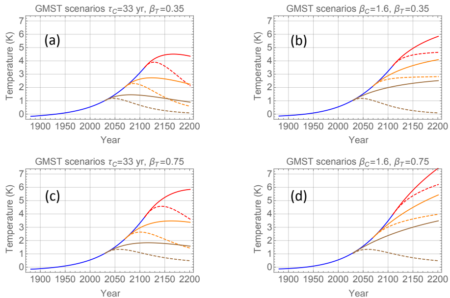
Figure 5. The evolution of the GMST for the CO 2 concentration scenarios shown in Fig. 4a and c. Panel (a): \tau_C = 33 years and \beta_T = 0.35 ; panel (b): \beta_C = 1.6 and \beta_T = 0.35 ; panel (c): \tau_C = 33 years and \beta_T = 0.75 ; panel (d): \beta_C = 1.6 and \beta_T = 0.75 .
