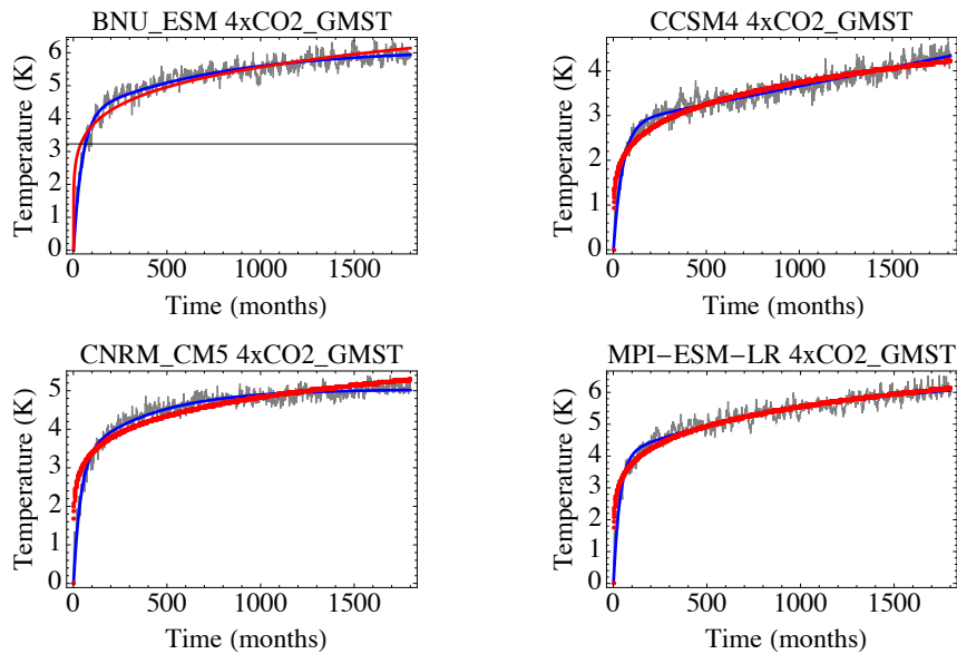
Figure D1. Blue curves: fit of the two-exponential response to the climate model responses to an abrupt quadrupling of atmospheric CO 2 concentration. Red curves: fit of the LRM-scaling response. The expressions fitted are found in the caption of Table 1 and the coefficients estimated are shown in this table.
