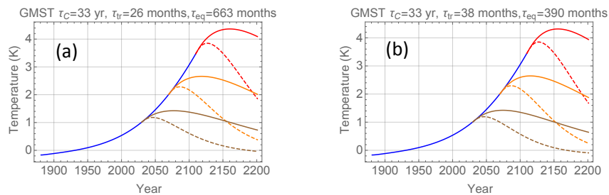
Figure D2. The evolution of the GMST according to the two-box model for the CO 2 concentration scenarios shown in Fig. 4a and c. Panel (a): \tau_C = 33 years and the two-box parameters for the GISS-E2-H given in Table 1. Panel (b): \tau_C = 33 years and the two-box parameters for the CNRM_CM5 model given in Table 1.
