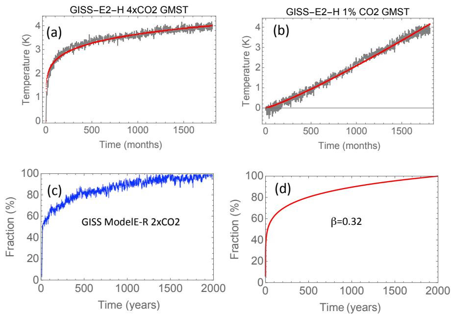
Figure C1. Panel (a): LRM response model fit c_1 t^{\beta_T/2} (red) to the GISS-E2-H model response to an abrupt quadrupling of atmospheric CO 2 (grey). The fit yields \beta_T = 0.32 . Panel (b): the LRM-response model solution c_2 t^{\beta_T/2+1} with \beta_T = 0.32 (red) and the GISS-E2-H model response to a 1% per year increase in atmospheric CO 2 concentration. Panel (c): the 2000-year response to a doubling of CO 2 in GISS ModelE-R as taken from Fig. 3 in Hansen et al. (2011). Panel (d): response to the same forcing in the LRM model with \beta_T = 0.32 .
