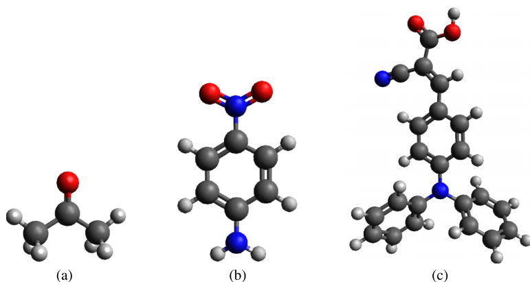
FIG. 2. Geometry of the molecules used in this paper. (a) Acetone. (b) PNA. (c) L0 dye.
