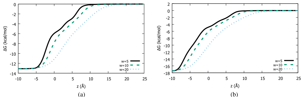
FIG. 5. Electrostatic energy profile for the water-vapor transfer of PNA molecule and L0 dye from Ref. 50. A droplet with R_0 = 20 Å, and interfacial width \tilde{w} as denoted in the legend (in Å) is considered. (a) PNA. (b) L0 dye from Ref. 50.
