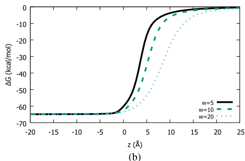
FIG. 3. Electrostatic energy profile for the water-vapor transfer of \text{Li}^+ and \text{Br}^- . A droplet with R_0 = 20 Å, and interfacial width \bar{w} as denoted in the legend (in Å) is considered. (a) \text{Li}^+ . (b) \text{Br}^- .
