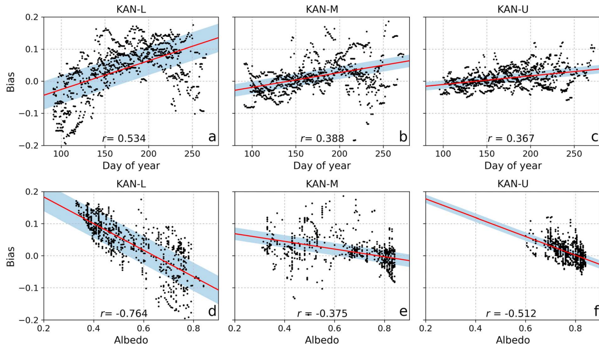
Figure 2. Relationship between MOD10A1 bias and (a–c) time since 1 April, and (d–f) albedo. The points represent every coincident observation from 2009 to 2016. All relationships are statistically significant to p < 0.01 .
