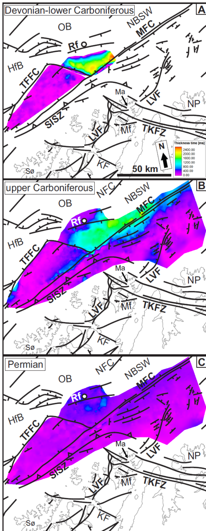
Figure 9: Thickness maps in milliseconds (ms) two-way time (TWT) of late Paleozoic sedimentary successions on the Finmark Platform and in the southwesternmost Nordkapp basin. Color scale in (a); a)
