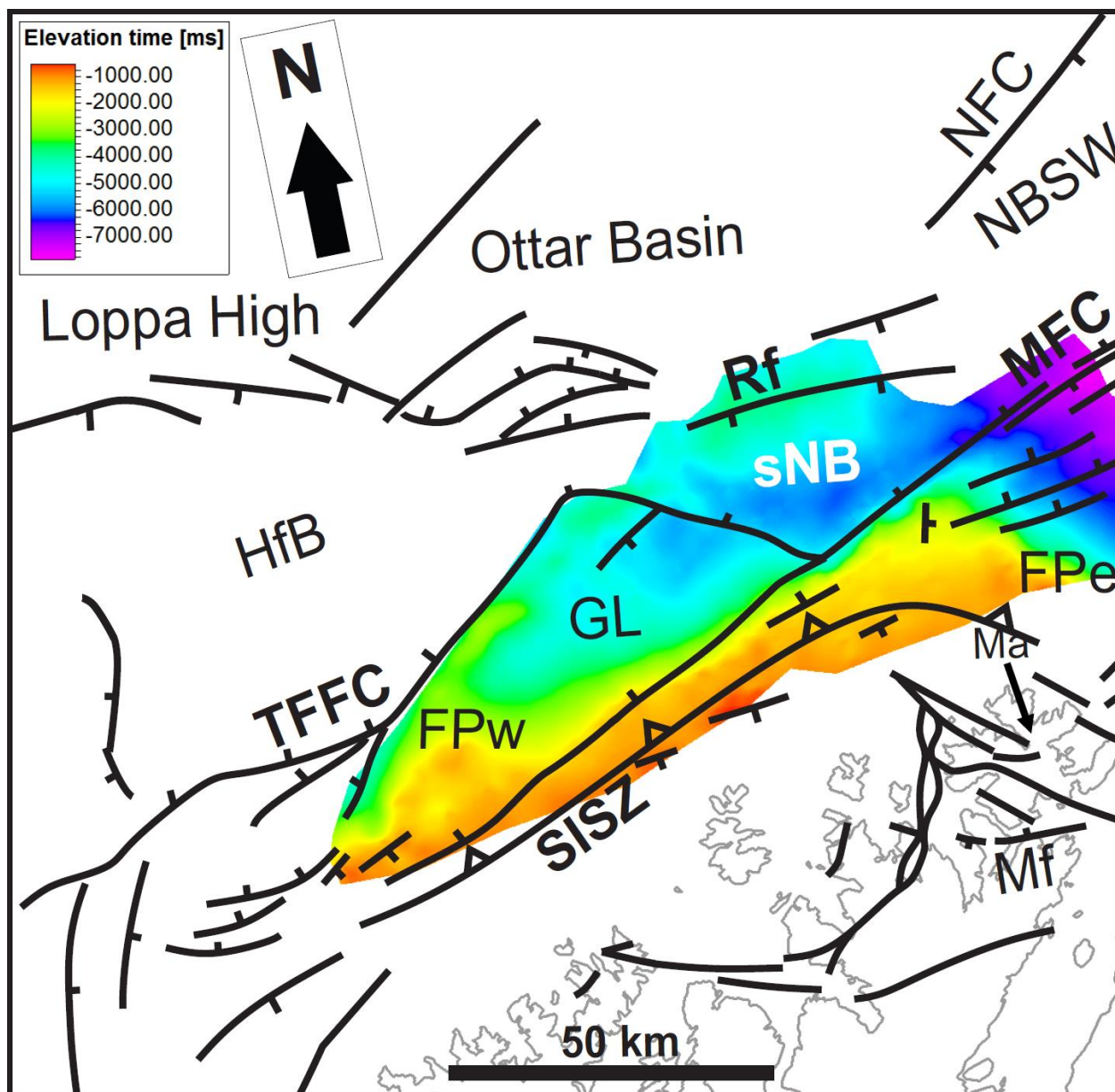
Figure 7: Time surface map of the top reflection of the SISZ and major brittle faults in the SW Barents Sea. Note the spoon-shaped depression formed by the SISZ on the Finnmark Platform west and southwesternmost Nordkapp basin, the abrupt change to a northeastward dip on the Finnmark Platform east, and the two narrow, NE-SW and ENE-WSW trending ridges in the footwall of the TfFc and of the Rolvsøya fault.
