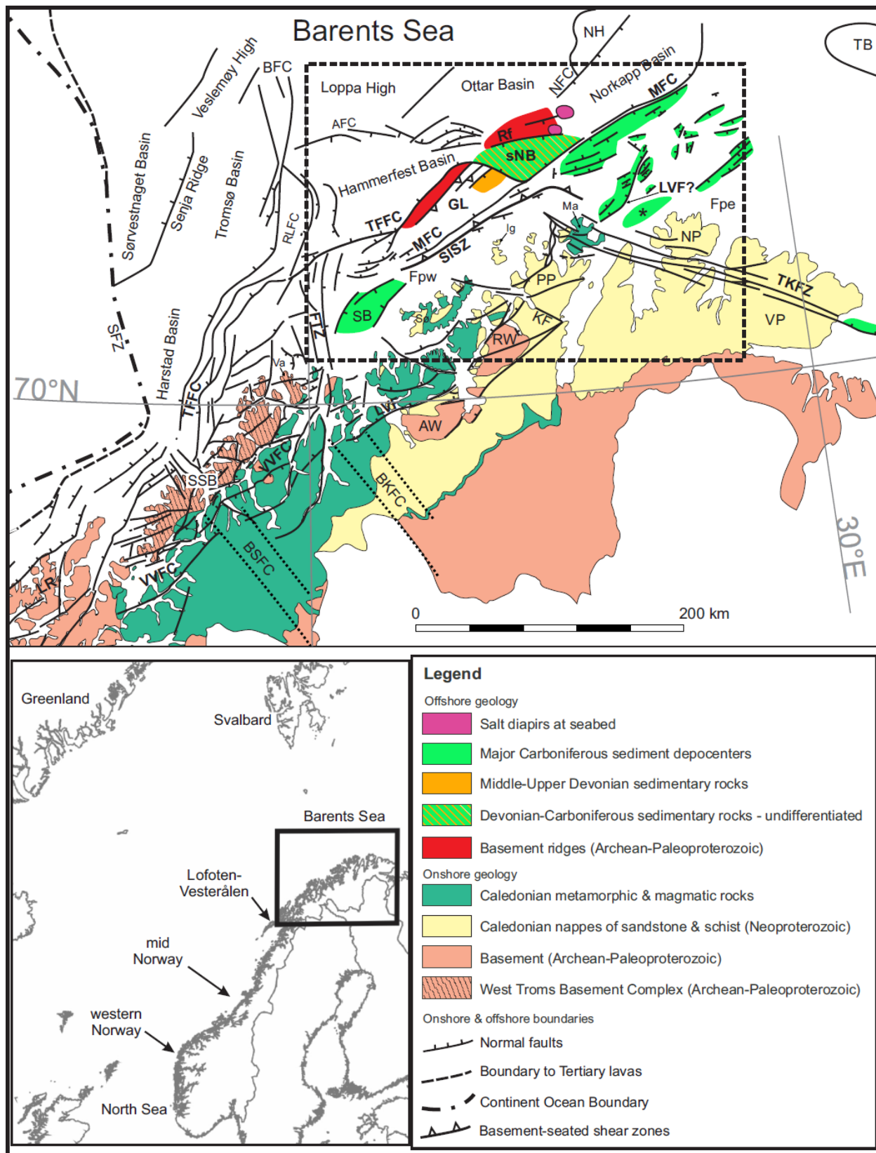
Figure 1: Regional structural map of the SW Barents Sea margin (based on Bergh et al. 2007, Faleide et al. 2008, Hansen et al. 2012 and Indrevær et al. 2013 and Koehl et al. submitted). The onshore geology is from the NGU and Ramberg et al. (2008). Dashed black frame locates Figure 2. The black star marks the location
