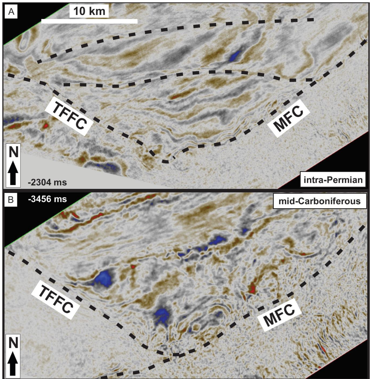
Figure 8: (a) Intra-Permian seismic time-slice within 3D seismic survey MC3D-MFZ02 in the southwesternmost Nordkapp basin. Dashed black lines correspond to interpreted brittle faults; (b) Seismic time-slice within 3D seismic survey MC3D-MFZ02 near the interpreted mid-Carboniferous reflection in the southwesternmost Nordkapp basin. Black dashed lines represent interpreted brittle faults. See Figure 2 for location.
