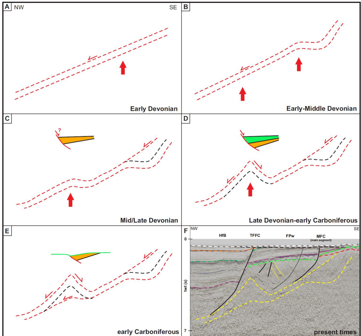
Figure 10: Evolutionary model explaining thickness variations along the SISZ. Note that the timing of (a) to (e) is tentative. Dashed red lines in (a) to (e) correspond to tectonically active portions of the SISZ whereas dashed black lines show inactive portions. Red lines in (c), (d) & (e) show presumed normal faults. Thick vertical red arrows indicate exhumation of basement rocks along the SISZ. The model is adapted to the geometry of the SISZ observed below the Finnmark Platform west (see f); a) Extensional reactivation (thin red arrow) of the SISZ in Early Devonian times. Rapid crustal thinning and possible erosion along the upper part of the SISZ triggers exhumation of basement rocks near the coasts of NW Finnmark (thick red arrow); b) In the Early-Middle Devonian, continued extension and erosion further thin the crust and exhume basement rocks in the footwall of the SISZ, leading the upper part of the SISZ to bow. Incremental crustal thinning due to continued extensional reactivation of the SISZ and continental erosion triggers exhumation of basement rocks along lower portions of the SISZ (left-hand side, thick red arrow); c) In Mid/Late Devonian times, bowed portions of the SISZ become inactive and excisement (i.e. upwards splaying; cf. Lister & Davis 1989) of the SISZ into its hanging-wall leads to thickening of the upper portion of the SISZ. Continued extension and erosion (i.e. crustal thinning) trigger bending of the lower part of the SISZ (thick red arrow) above which brittle normal faults may have formed and localized the deposition of Devonian sedimentary deposits (orange); d) Further exhumation of basement rocks along lower portions of the SISZ in the Late Devonian-early Carboniferous leads to extreme bending of the SISZ, to antithetic top-to-the-SE extensional faulting, and to early Carboniferous syn-tectonic sedimentation (green); e) Towards the end of the early Carboniferous, the lower portion of the SISZ is thickened due to incisement (i.e. downward splaying; cf. Lister & Davis 1989) of the SISZ into bow-shaped portions in its footwall. Core complex exhumation ceased in the Serpukhovian and a major sea-level fall exposed the Finnmark Platform to continental erosion (green line representing the mid-Carboniferous reflection); f) Present times seismic expression of thickness
