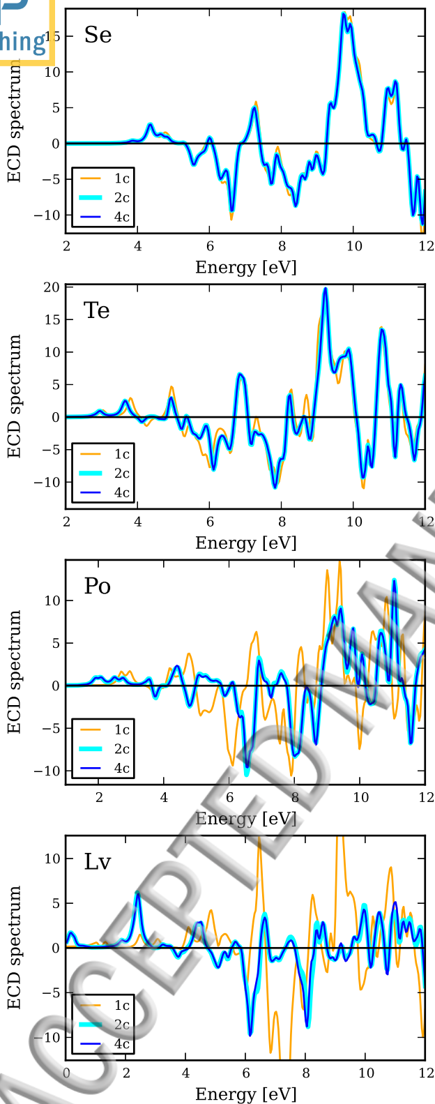
FIG. 3: The comparison of 1c, 2c (X2C) and 4c (DC) ECD spectra (in atomic units) of dimethylchalcogeniranes computed using PBE functional with RI-J acceleration. The corresponding spectra are labelled by the chemical symbol of the heteroatom. ECD spectra of lighter analogues and all ORD spectra can be found in the Supplementary Material.
