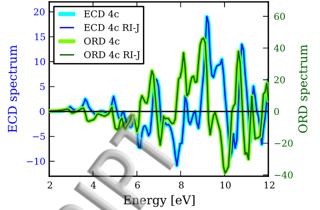
FIG. 2: The comparison of 4c ECD and ORD spectra (in atomic units) of Te-based system calculated with and without the RI-J acceleration. The simulation proceeded for 15000 time steps of length 0.15 au.
