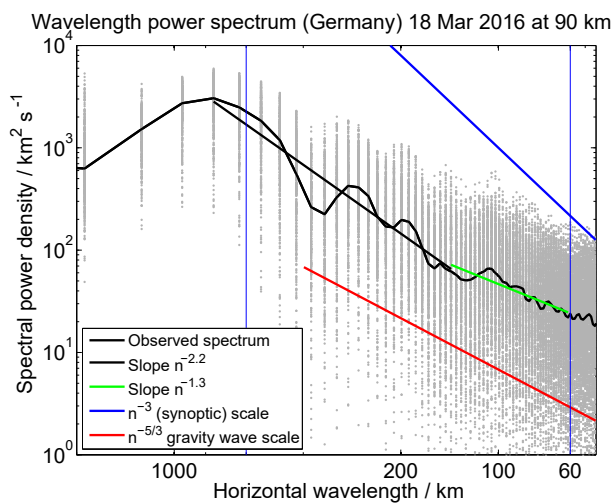
Figure 15. Horizontal wavelength spectra and estimated slopes to identify the transition from the mesoscale GW to the synoptic scale.
