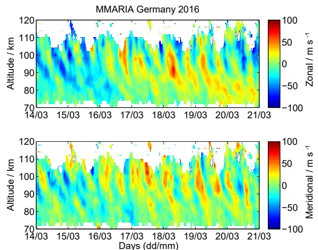
Figure 11. Overview of zonal and meridional wind components applying the standard wind analysis to the MMARIA network during the March 2016 campaign.
