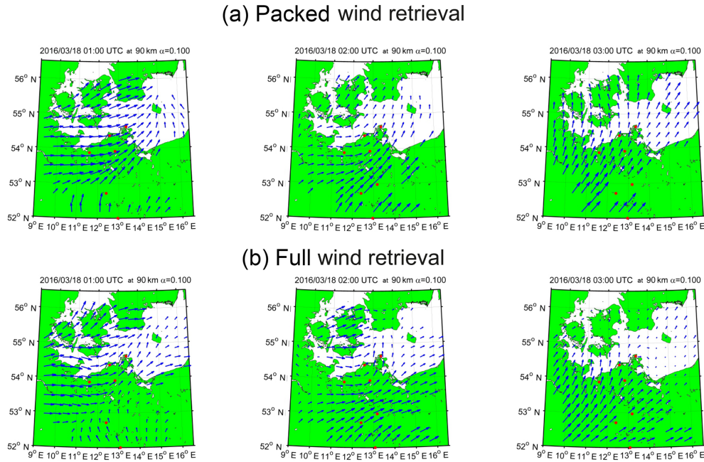
Figure 7. Comparison of wind retrievals. Panel (a) shows the solutions of the “packed wind retrieval”. Panel (b) shows the same time and altitudes for the “full wind retrieval”.
