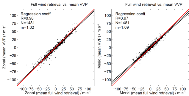
Figure 13. Scatter plots of mean zonal and meridional winds obtained from the full wind retrieval and VVP. The mean is computed as average over the domain area.
