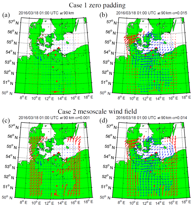
Figure 6. Comparison of wind field solution in dependence of the background mesoscale solution. (a, b) Test case with zero padding: first (a) and final iteration (b). (c, d) Test case with mesoscale wind field (obtained from the data): first (c) and final iteration (d).
