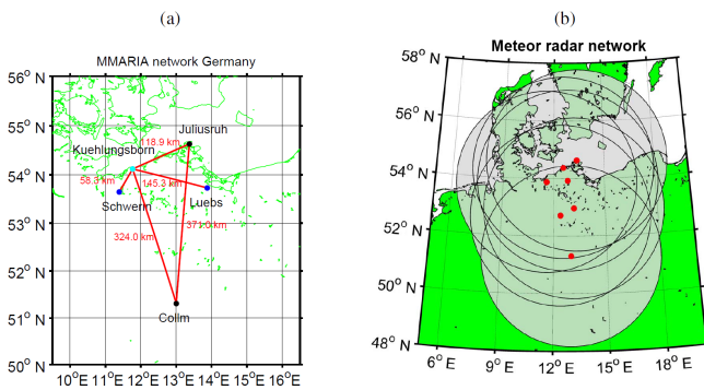
Figure 10. (a) Schematic view of multi-static network during the campaign in March 2016. (b) Geographic map of different viewing geometries (red points). The shaded areas label a circle of 300 km in diameter around each center of radial velocity measurements.
