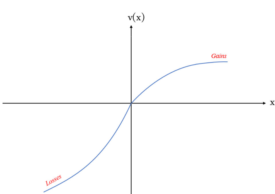
Figure 3 - Value function
