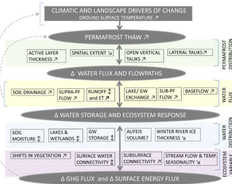
Figure 1. A sketch of impacts and responses of permafrost thawing on water fluxes and distribution. The symbols of \Delta , \nearrow , \searrow , \downarrow , and ? denote change, increase, decrease, variation, and unknown changes, respectively. Modified from [25].
