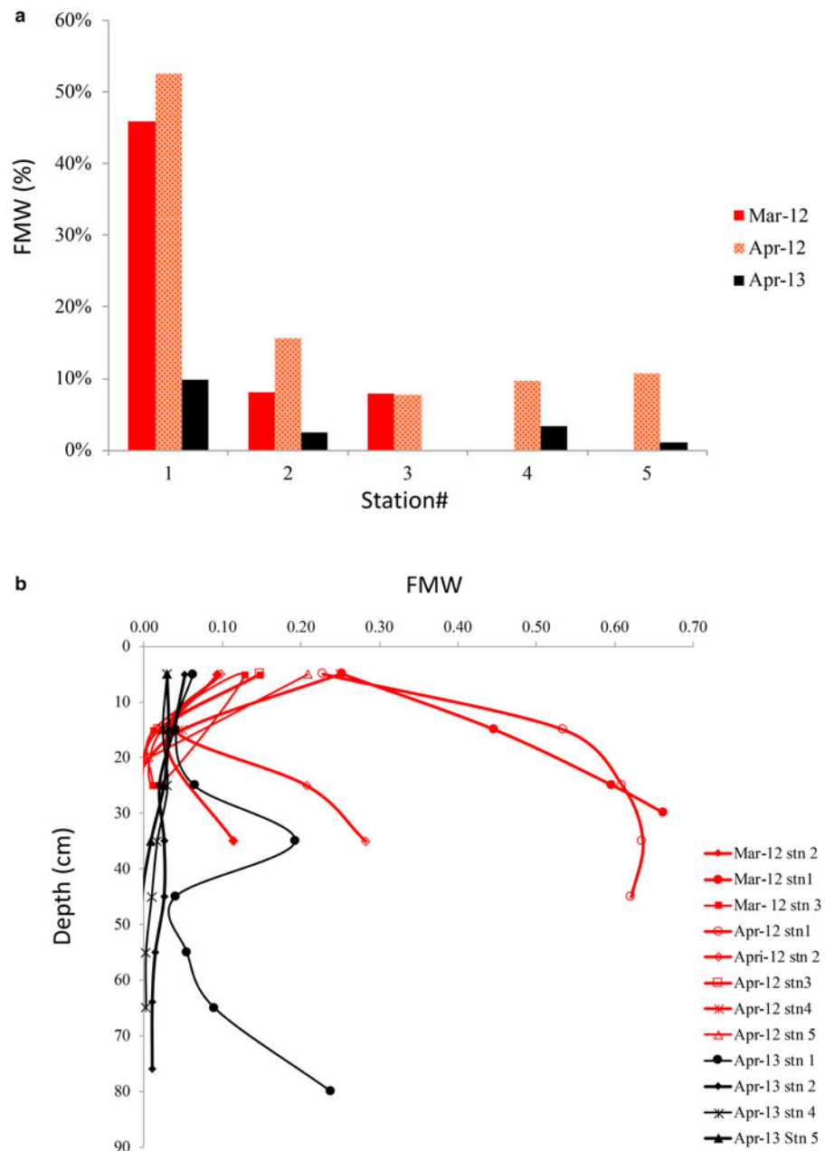
Fig. 6. The fraction of meteoric water (FMW) in sea ice as (a) integrated freshwater content (FMW, %) in the sea ice at the five stations, from the glacier front (station #1) to station #5 (8 km on the x-axis) in Tempelfjorden in March 2012 (red), April 2012 (red dotted) and April 2013 (black), and (b) the vertical distribution of FMW (as fractions) in the sea ice for each station in March 2012 (red, closed symbols), April 2012 (red, open symbols) and April 2013 (black).
