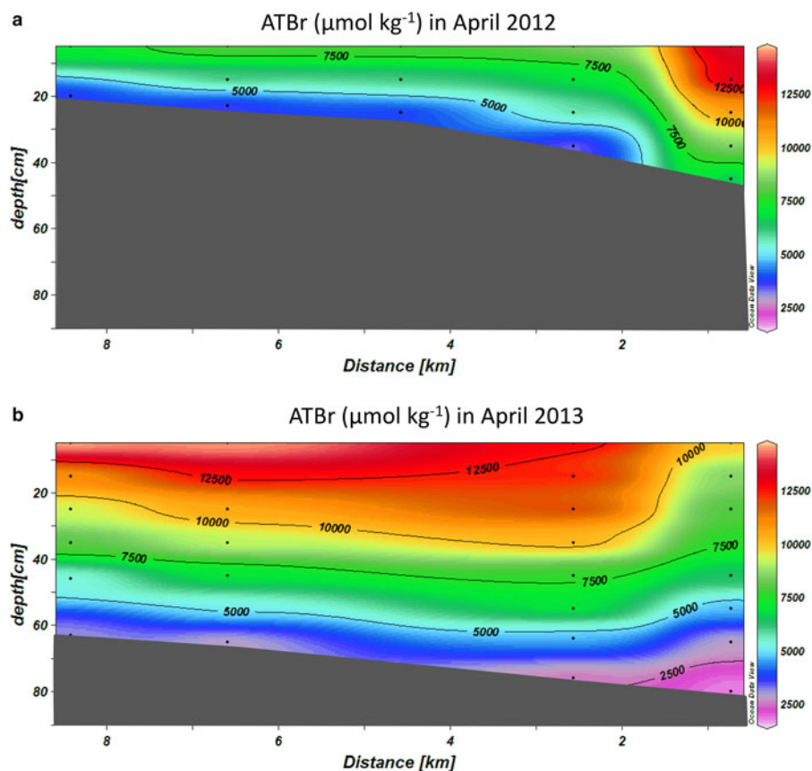
Fig. 9. Vertical profiles of brine-volume corrected total alkalinity ( A_{\text{TBV}} , \mu\text{mol kg}^{-1} ) of the chemical variables in April 2012 and April 2013 along the section in the fjord, from the glacier front (GF, station #1) to station #5.
