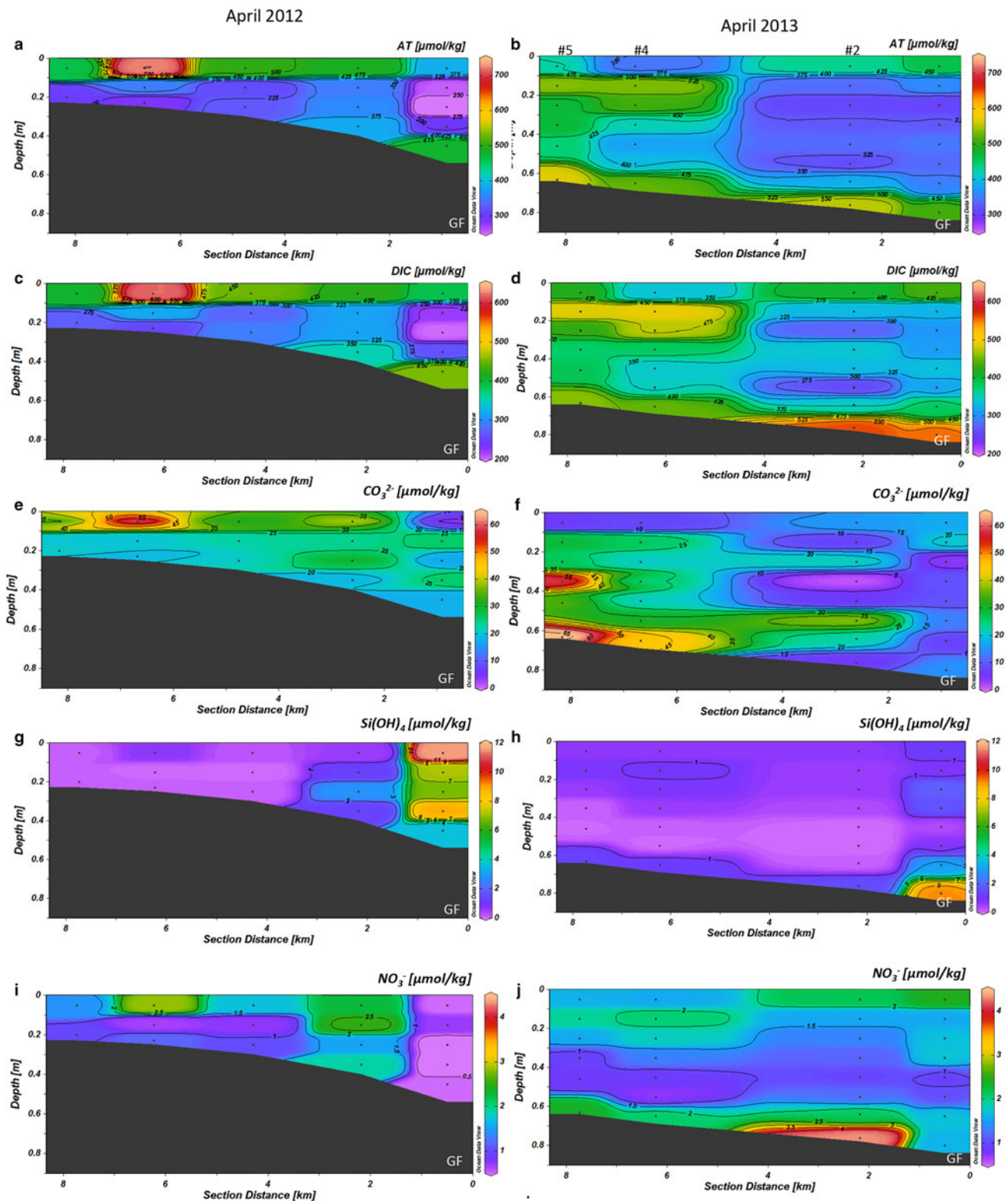
Fig. 4. Sea-ice bulk properties of the chemical variables in April 2012 and April 2013 along the section from the glacier front (GF, 0 km on x -axis, station #1) to station #5 (8 km on the x -axis): (a, b) total alkalinity ( A_T , \mu\text{mol kg}^{-1} ), (c, d) total dissolved inorganic carbon (DIC, \mu\text{mol kg}^{-1} ), (e, f) carbonate ion concentration ( [\text{CO}_3^{2-}] , \mu\text{mol kg}^{-1} ), (g, h) silicate concentration ( [\text{Si}(\text{OH})_4] , \mu\text{mol kg}^{-1} ), and (i, j) nitrate ( [\text{NO}_3^-] , \mu\text{mol kg}^{-1} ). Dots denote the sampling depth in the sea ice. The dark field shows the under-ice water and the ice-water boundary. Note that station #3 was not sampled in 2013, thus the values between stations #2 and #4 are extrapolated and should be interpreted with caution.
