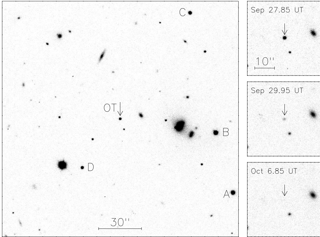
Fig. 1. Left panel: An R-band finding-chart for GRB 000926 centred on the position of the OT (marked with an arrow). Also marked are the four secondary calibration stars A–D used to transform the relative PSF-photometry onto the standard system. The photometric properties of the stars are given in Table 1. Right panels: Three smaller R-band images centred on the OT at three different epochs showing the decline of the OT.
