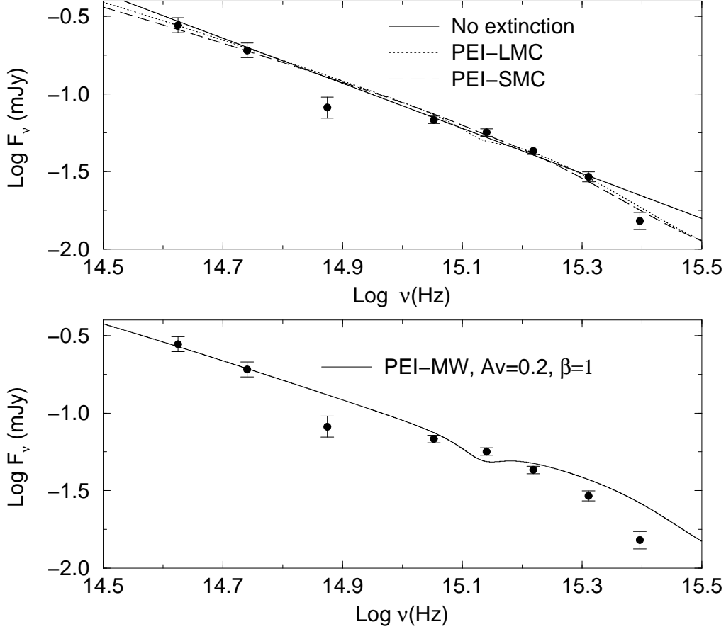
Fig. 3. The observed specific flux F_\nu vs. the rest-frame frequency \nu normalised to Sep 27.9 UT. The spectral energy distribution of the afterglow from K to U is clearly curved. In the upper panel we show that this curvature can be well fitted by an underlying \beta = 1 power-law SED with a SMC or LMC extinction law with A_V=0.2 . In the lower panel we show that the MW extinction law is inconsistent with the data.
