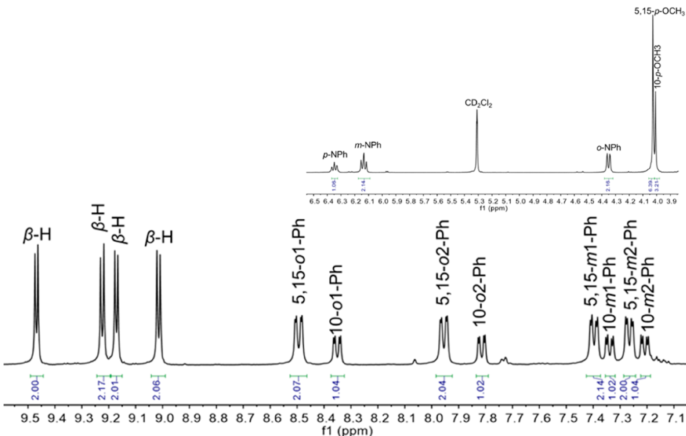
Figure 1. Representative ^1\text{H} NMR spectrum: \text{Re}[\text{TpOCH}_3\text{PC}](\text{NPh}) .
