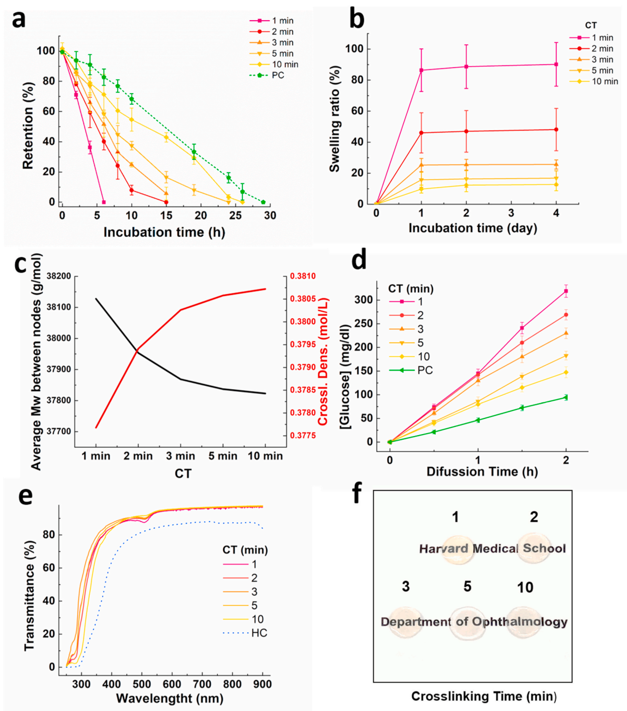
Fig. 3. Structural and optical properties of GELGYM. a) Collagenase induced degradation rate of GELGYM hydrogels (FD of 175% and 22.5% w/v) with varying CT from 1 to 10 min as a function of incubation time ( T = 37^\circ\text{C} and 5% \text{CO}_2 ). b) Swelling ratio of GELGYM hydrogels (FD of 175% and 22.5% w/v) with varying CT from 1 to 10 min. c) Crosslinking density and an average molecular weight between nodes of gelatin-based hydrogels at different crosslinking times. d) Glucose permeability and e) optical transmittance of GELGYM hydrogels (FD of 175% and 22.5% w/v) with varying CT from 1 to 10 min in the range on 250–850 nm. f) GELGYM transparency images at different crosslinking times. PC: porcine cornea; HC: human cornea.
