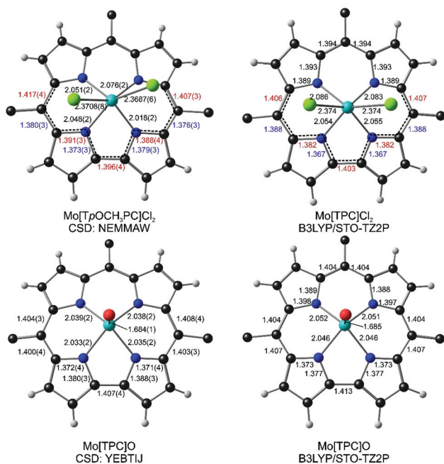
Fig. 1 Selected distances in the X-ray structures of Mo[TP 3 OCH 3 PC]Cl 2 and Mo[TPC]O and the DFT (B3LYP/STO-TZ2P) optimized geometries of Mo[TPC]Cl 2 and Mo[TPC]O. Parts of the corrole skeleton exhibiting bond length alternation are indicated with dashed lines and alternate longer and shorter bonds therein are indicated in red and blue, respectively.
