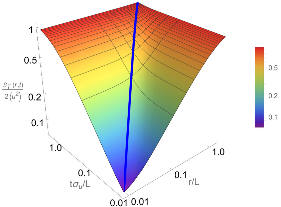
FIGURE 15. Model results for the space-time varying structure function. Since the model applies only to the inertial subrange, the figure is restricted to r \geq \eta_0 and t \geq \tau_K . A solid blue line gives r = \sigma_u t .
