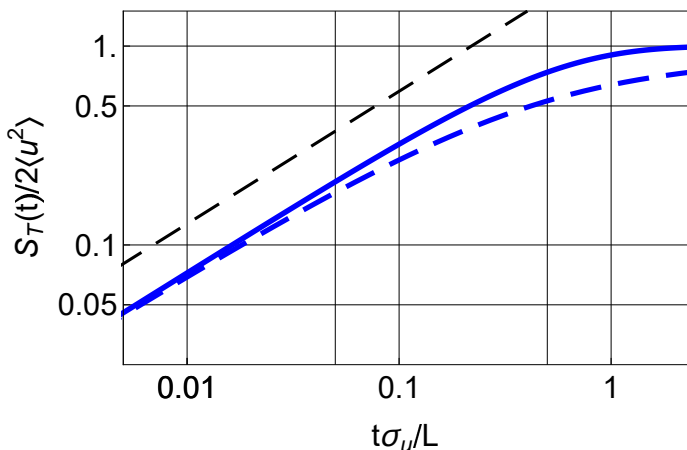
FIGURE 14. The temporal variation model structure function for varying normalized time separations. For reference we have a thin dashed line giving the slope of t^{2/3} . The heavy dashed line gives the result for filtered advection velocities.
