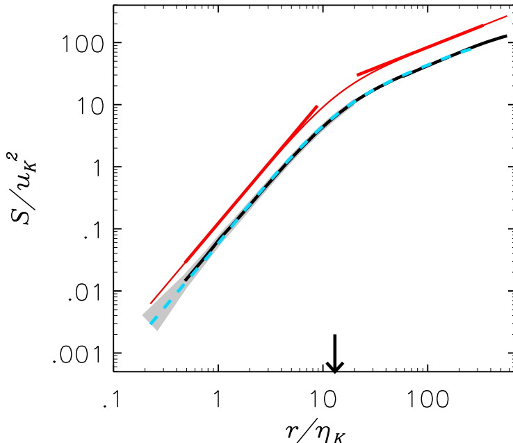
FIGURE 1. The numerically obtained normalized longitudinal structure function \mathcal{S}(r)/u_K^2 \equiv \langle (u_{\parallel}(\boldsymbol{\xi}, t) - u_{\parallel}(\boldsymbol{\xi} + \mathbf{r}, t))^2 \rangle / u_K^2 , shown on a double logarithmic scale for varying normalized separation r/\eta_K , with \eta_K = (\nu^3/\epsilon)^{1/4} being the Kolmogorov length scale, see also Pécseli et al. (2020). The Kolmogorov velocity u_K = (\nu\epsilon)^{1/4} is used for normalization. Results from the two simulations (I and II) are shown with blue dashed and black full lines, respectively. Analytical results are shown for the inertial and viscous subranges by the slopes of the red lines with r^{2/3} and r^2 , respectively. For clarity of presentation, the two slopes as well as an empirical analytical approximation (thin red line) have been offset vertically by a factor 2. A vertical arrow indicates the "cross-over" length between the two subranges at r = \eta_0 . The uncertainty at small separations is indicated by a grey shading. This shading is representative also for the following figures 2, 3, 8, and 9.
