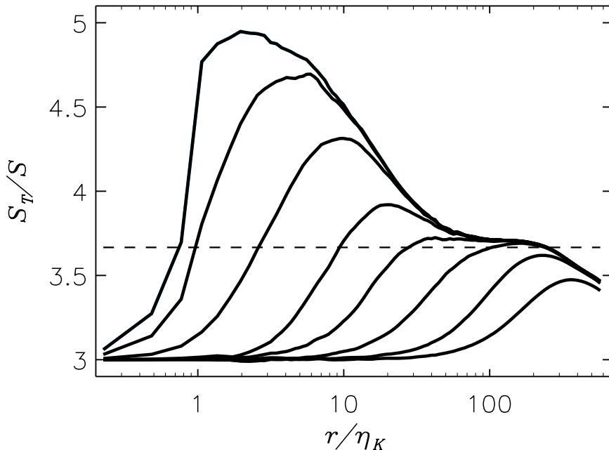
FIGURE 5. The ratio \mathcal{S}_T(r,t)/\mathcal{S}(r,t) derived from the longitudinal and transverse structure functions for dataset II is shown here on a linear vertical scale for selected times t/\tau_K = 0.0, 0.04, 0.35, 0.70, 2.51, 6.84, and 17.45 . For r > \eta_0 we find a plateau developing near 11/3 shown by a dashed line, while we for r \rightarrow 0 with t = 0 find a saturation at the level 5. The curves are uncertain for r < \eta_K because only few samples for the estimation of the structure functions are found at these small separations. The noise for small r seen in figure 4 is found also here.
