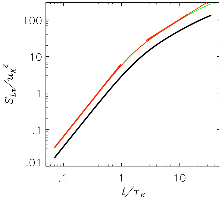
FIGURE 6. Estimate for the normalized Lagrangian structure function \mathcal{S}_{Lx}(t)/u_K^2 using dataset II, shown as a function of normalized time variable t/\tau_K with logarithmic scales on both axes. Full red reference lines give the slopes for t^2 and t . The thin red curve gives the empirical transition between the viscous and the inertial ranges corresponding to the transition parameter p = 5/2 , see Appendix B. The underlying green curve illustrates the corresponding analytical model for the transition from the universal range to the asymptotic limit for a transition parameter p = 2 .
