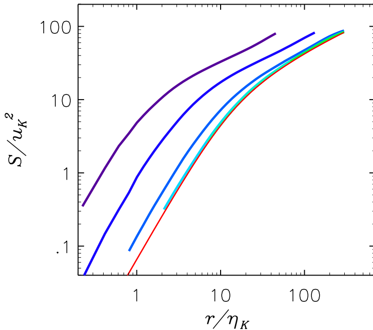
FIGURE 8. Sampling of the normalized structure function \mathcal{S} along lines r = Vt for V/u_{rms} = 0.1, 0.3, 1, 3, 10 and 100 from figure 2 (dataset I). A thin red line give the analytical approximation (B 1) for \mathcal{S}(r) . The results for V/u_{rms} = 3, 10 and 100 are hardly distinguishable with the given line thickness. The top curve is for V/u_{rms} = 0.1 with V increasing down.
