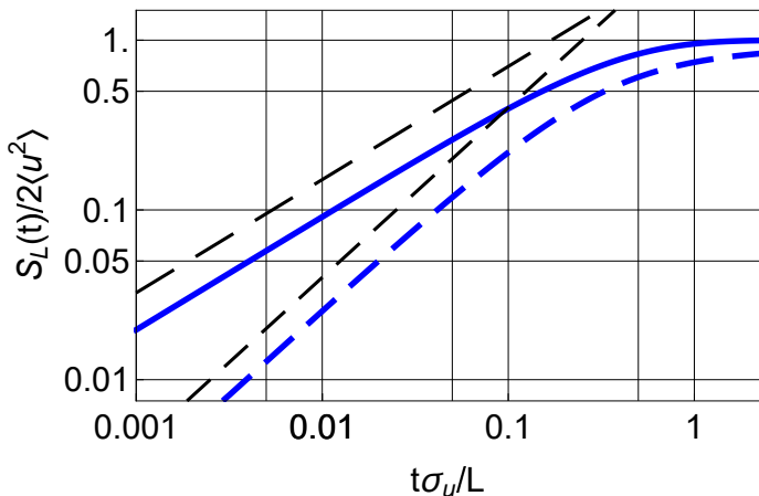
FIGURE 18. Model results for the Lagrangian structure function. The full line gives the result found by Wandel & Kofoed-Hansen (1962), the thick dashed line is the one suggested in the present analysis. Two thin dashed lines gives the reference slopes of t^{2/3} and t , respectively.
