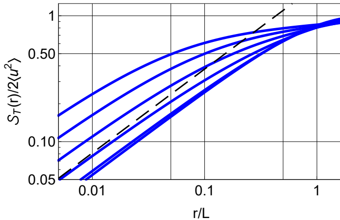
FIGURE 17. Model results (in a double logarithmic presentation) for samples of the Taylor hypothesis applied to the filtered version of the KWH structure function using V/\sigma_u = 1/8, 1/4, 1/2, 1, 5/2 , and 10 from top to bottom, to be compared with figures 8 and 9. A dashed line gives the slope of r^{2/3} for reference.
