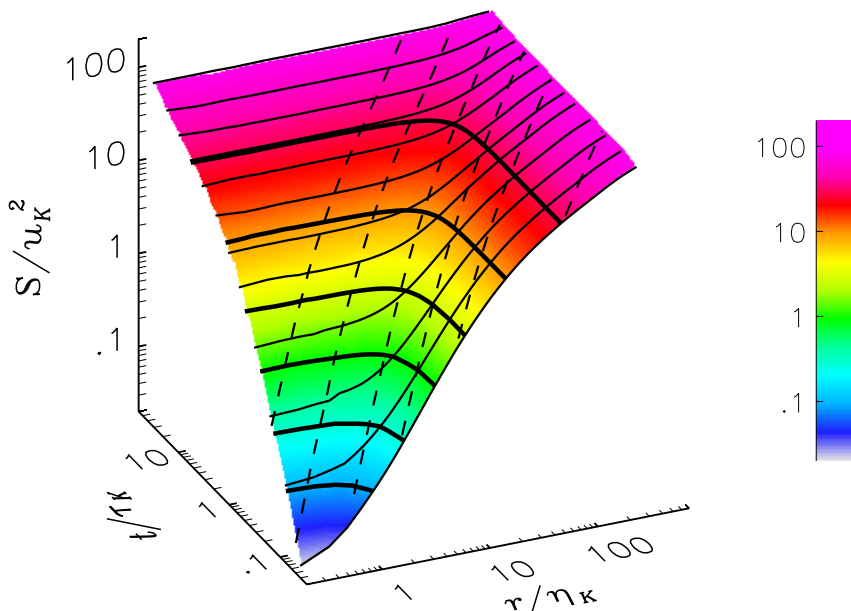
FIGURE 2. Estimate for the normalized longitudinal structure function \mathcal{S}(r, t)/u_K^2 using dataset I, shown as a function of normalized variables r/\eta_K and t/\tau_K with logarithmic scales on all axes. Full black lines are for the levels \{0.1, 0.3, 1, 3, 10, 30\} , the dashed lines for normalized velocities V/u_{rms} = \{0.1, 0.3, 1, 3, 10, \dots, 100\} . These lines will be parallel when projected on the r-t plane for logarithmic scales. The time separation axis begins at t = 0.02\tau , the spatial separations at r = 0.4\eta_K . Thin black parallel lines are given for selected t -values and serve only as a guide for the eye.
