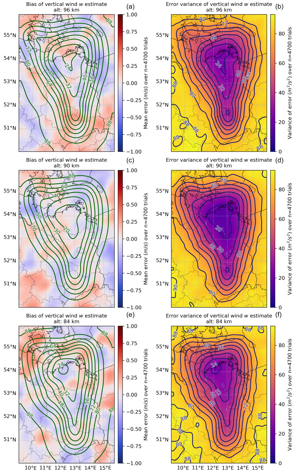
Figure 4. Statistics of the vertical wind estimator error relative to the simulated truth. Each panel shows the bias (a, c, e) or error variance (b, d, f) as a function of latitude and longitude averaged over n = 100 trials at each of 47 measurement geometries taken throughout 1 d. Contours on the bias plots give the posterior predictive variance (in m^2 s^{-2} ), indicating more confidence in the central areas where the bias also tends to be a little lower. Contours on the error variance plots correspond to the sample error variance (matching the coloring).
