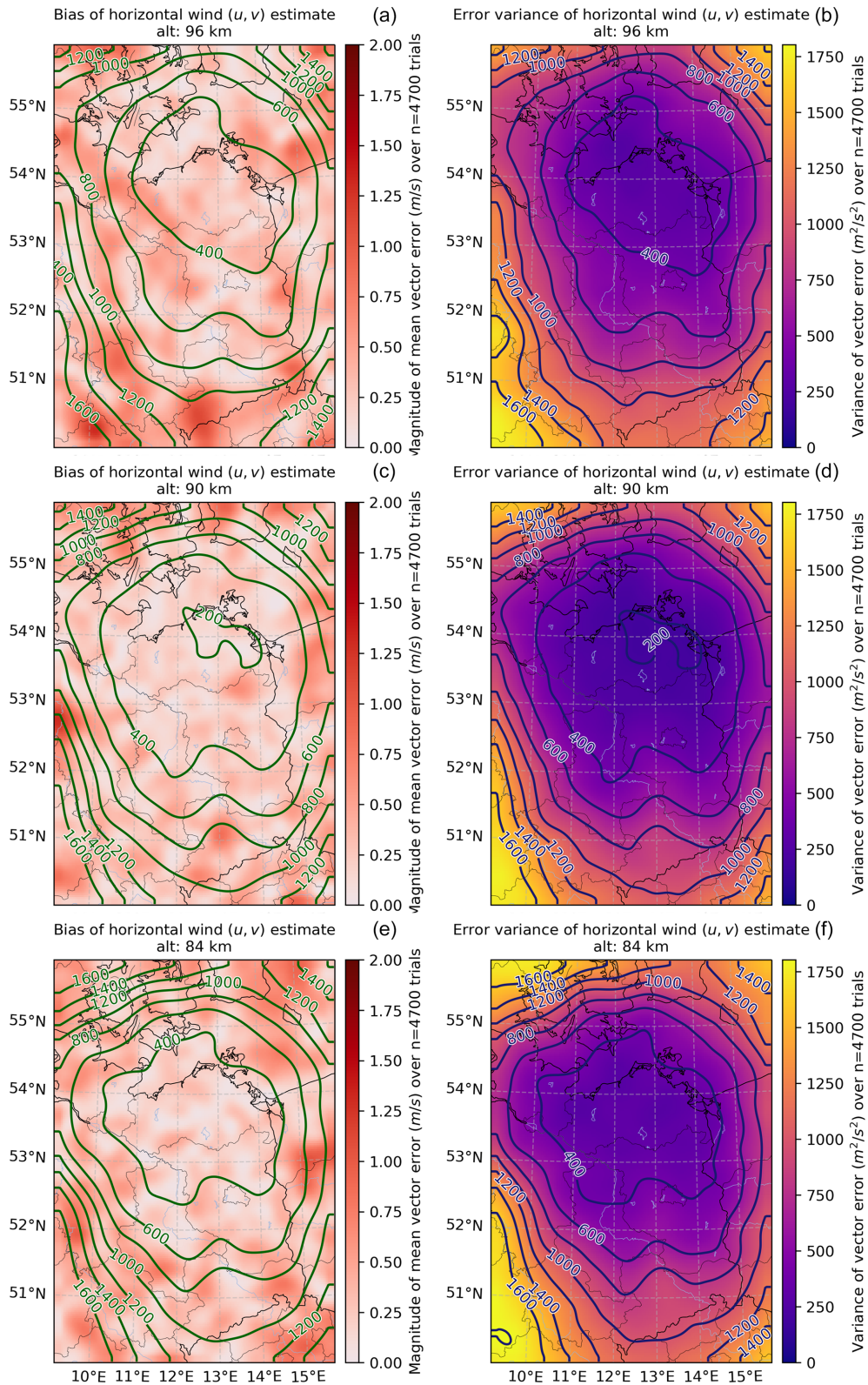
Figure 3. Statistics of the horizontal wind estimator error relative to the simulated truth. Each panel shows the bias ( a , c , e ) or error variance ( b , d , f ) as a function of latitude and longitude averaged over n = 100 trials at each of 47 measurement geometries taken throughout 1 d. Contours on the bias plots give the posterior predictive variance (in \text{m}^2 \text{s}^{-2} ), indicating more confidence in the central areas where the bias also tends to be a little lower. Contours on the error variance plots correspond to the sample error variance (matching the coloring).
