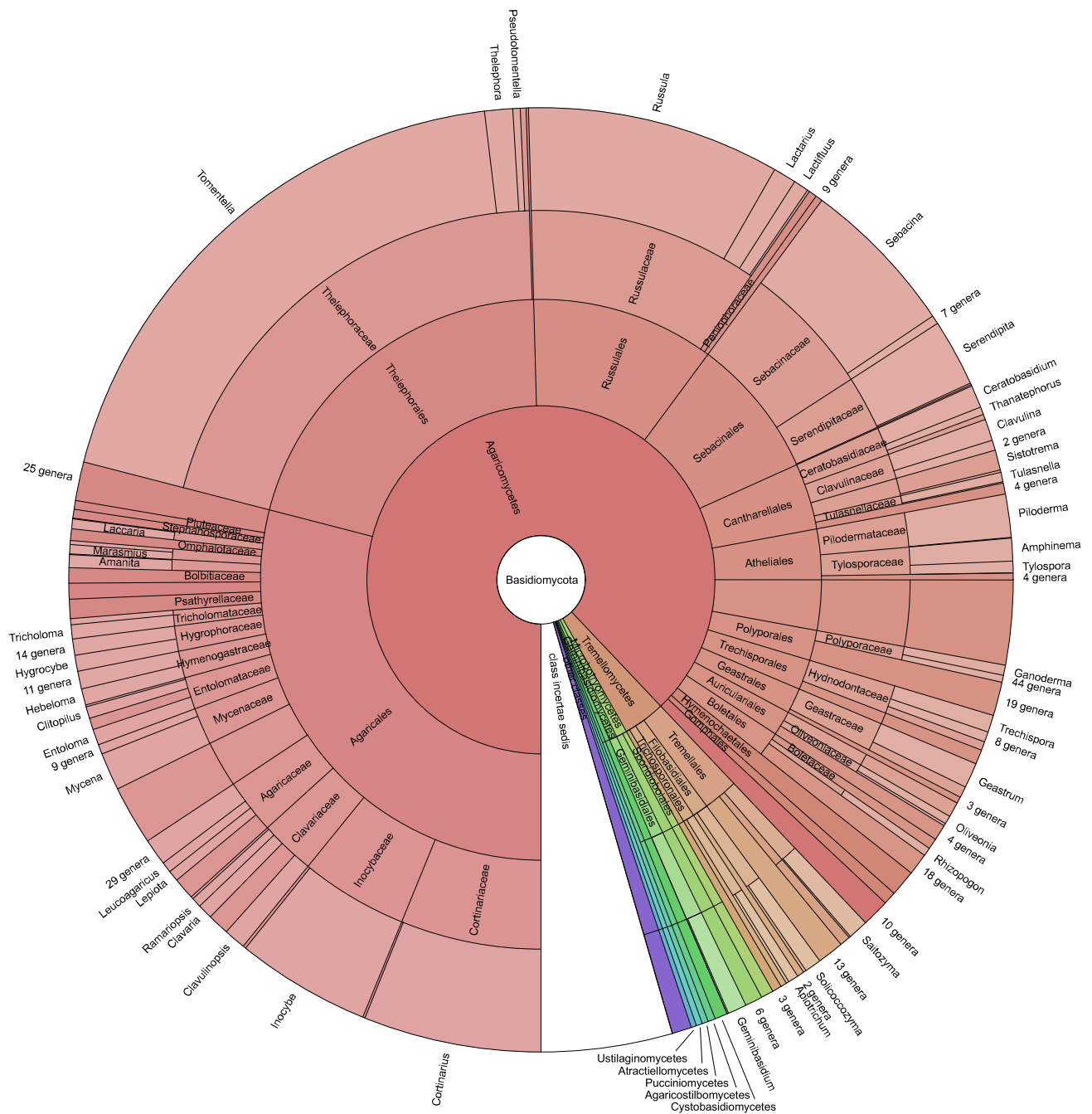
Fig. 4 Taxonomic profile of the Basidiomycota components in the samples based on a Krona chart. The figure can be interactively expanded at https://doi.org/10.15156/BIO/1436941
