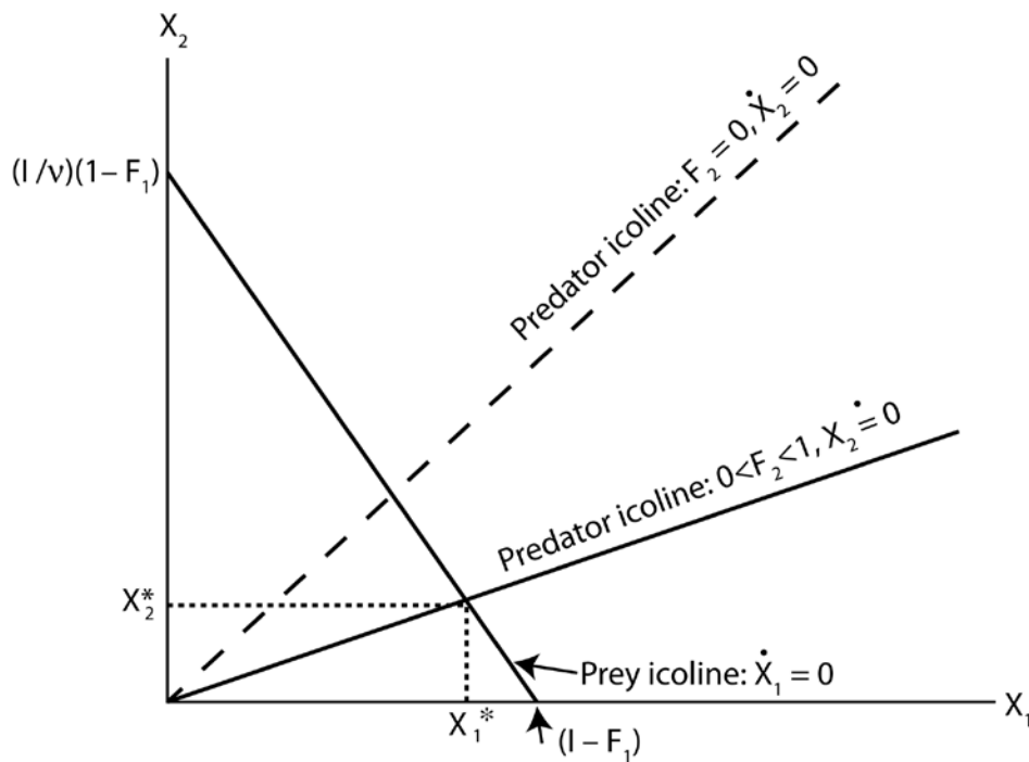
Figure 9.6. Phase diagram for a predator-prey model.
