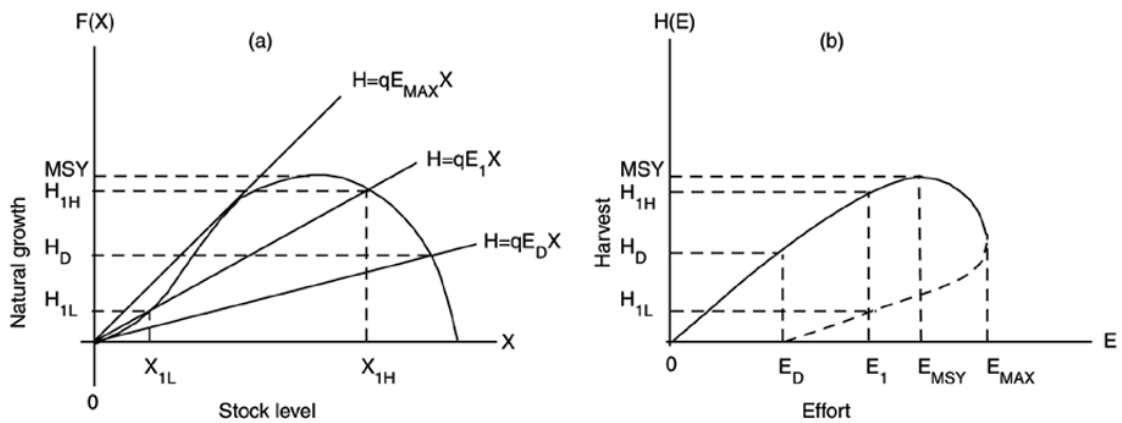
Figure 2.4. The natural growth curve and sustainable yield as a function of effort in the case of depensation.
