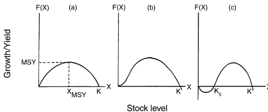
Figure 2.1. Growth curves with (a) compensation, (b) depensation, and (c) critical depensation.
