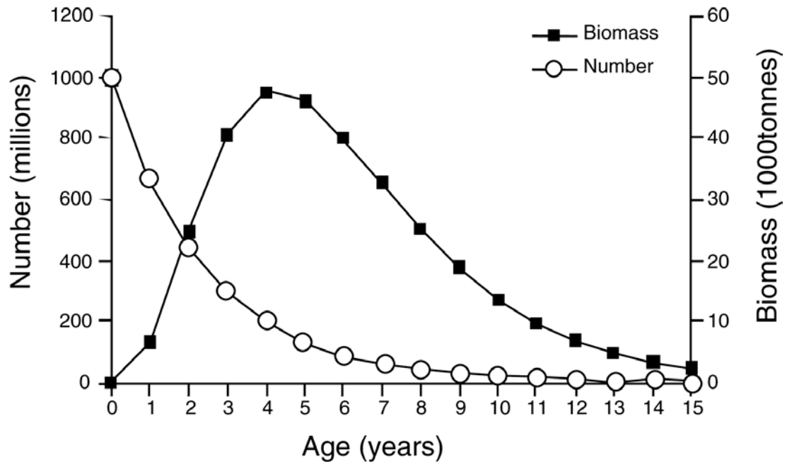
Figure 8.3. The decline in number of fishes and the rise and decline of biomass in a given cohort of mackerel, without fishing. Parameters used are N(0) = 1 billion, M = 0.4 and growth parameters as in figure 8.2.
