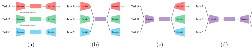
Fig. 2. Common MTL workflows for dense prediction tasks. The data modalities of the input are different: (a) The different tasks have separate networks, which are linked through soft parameter sharing . Note, without soft parameter sharing, (a) depicts the standard multiple single-task learning. (b) The different tasks have independent encoders and decoders but share the same network backbone (in purple), which is also known as hard parameter sharing . The data modalities of the input are identical: (c) Each task has independent output, which requires an independent decoder. (d) The tasks can share the same decoder.
