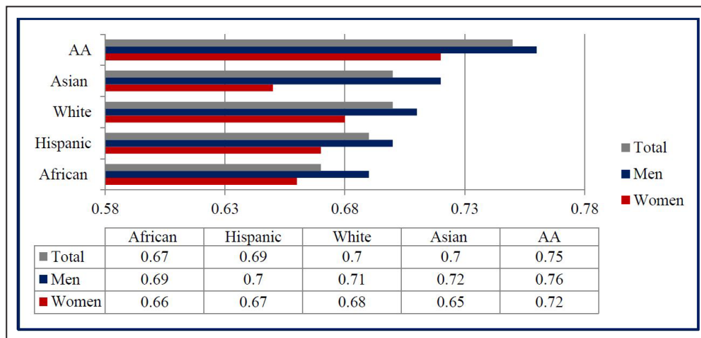
Figure 1. Adjusted means of common CIMT in mm (with 95% CIs) across the racial and ethnic groups in the USE-IMT and AWI-Gen collaborative study’s combined sample.
