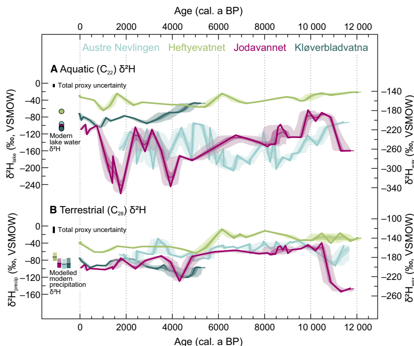
Fig. 5. Leaf wax \delta^2\text{H} values (right axis) and leaf wax \delta^2\text{H} converted to lake water or precipitation \delta^2\text{H} values (left axis) for aquatic ( \text{C}_{22} ) (A) and terrestrial ( \text{C}_{28} ) (B) plant n -alkanoic acids from Heftyevatnet, Jodavannet, Austre Nevlingen, and Kløverbladvatna, Svalbard. Bold line: measured values plotted on the median age of each sample; fine line: median value of all age model iterations; light and dark shading: 1\sigma and 2\sigma age model uncertainty, respectively. The vertical black bars represent the total proxy uncertainty and include analytical and conversion uncertainties. Modern summer lake water \delta^2\text{H} values (circles) and modelled precipitation \delta^2\text{H} values (bars; representing ranges between weighted mean annual (black line) and maximum and minimum monthly precipitation) from the Online Isotopes in Precipitation Calculator (OIPC; Bowen et al. 2005; IAEA/ WMO 2019; Bowen 2021) are plotted for comparison.
