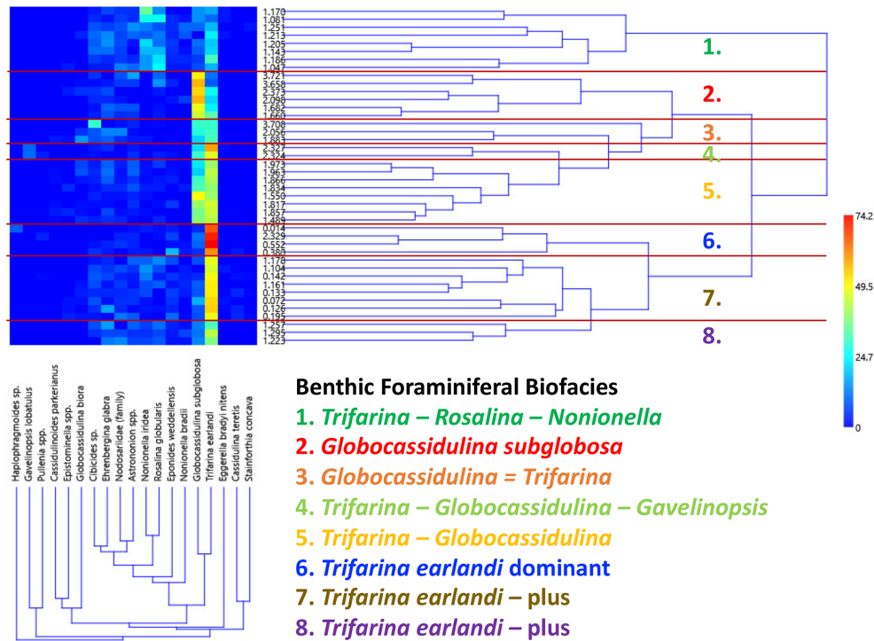
Figure 7. Q-mode and R-mode combined cluster analysis using PAST and the Bray–Curtis similarity index. This analysis includes samples with 40 or more specimens ( N=42 ). The two dominant taxa are Trifarina earlandi and Globocassidulina subglobosa . See the discussion in the text.
