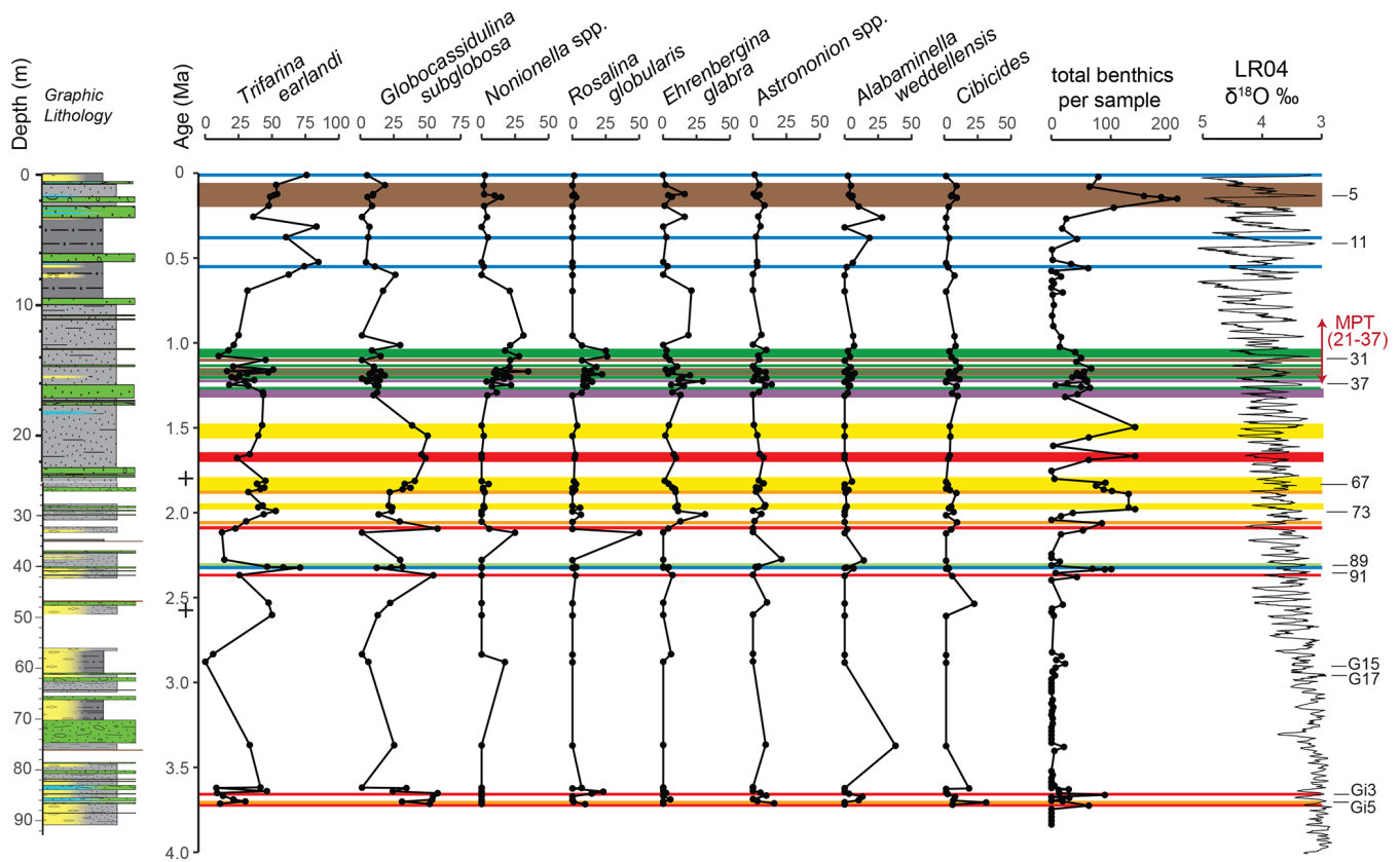
Figure 8. Benthic foraminiferal biofacies at Site U1523 based on Q-mode and R-mode cluster analysis and the Bray–Curtis similarity index. Only includes samples with 40 or more specimens ( N = 42 ). Color-coded horizontal bars represent biofacies defined in Fig. 7. Note the major change in benthic foraminiferal biofacies after \sim 1.5 Ma: from Globocassidulina subglobosa -dominant or co-dominant biofacies (red, orange, yellow) to Trifarina earlandi -dominant biofacies (blue, brown, purple, green), reflecting the increasing influence of the Antarctic Slope Current in the mid to Late Pleistocene. The graphic lithology is from Gales et al. (2023). The two + symbols in the age column mark the position of the two magnetic reversals that help define the age model used for Site U1523.
