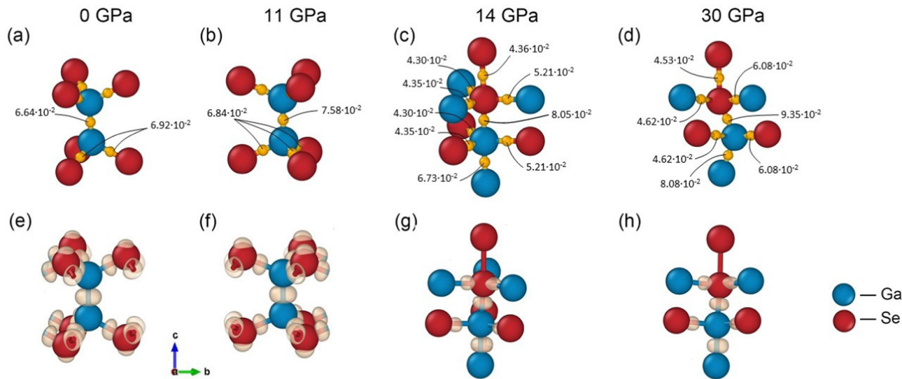
Fig. 4 Bader analysis showing the bond critical points with the value of electron density in e\text{-bohr}^{-3} at each of them and charge density difference (CDD) distribution for GaSe.
