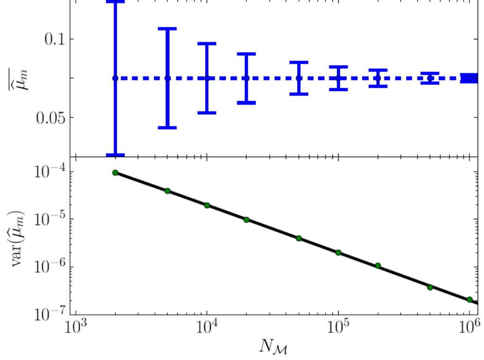
FIG. 22. Sample mean (upper panel) and variance (lower panel) of the estimators \{\widehat{\mu}_m\} computed from the synthetic time series with \gamma = 0.1 . The dashed line in the upper panel is \widehat{\mu} computed with N data points, the black line in the lower panel is given by Eqn. (59).
