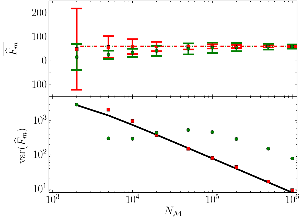
FIG. 6: Sample mean (upper panel) and variance (lower panel) of the estimators \{\widehat{F}_{\Gamma, m}\} (red square) and \{\widehat{F}_m\} (green circle) computed from the synthetic time series with \gamma = 0.1 . The dashed (dotted) line in the upper panel is \widehat{F}_{\Gamma} ( \widehat{F} ) computed with N data points, the black line in the lower panel is given by Eq. (16).
