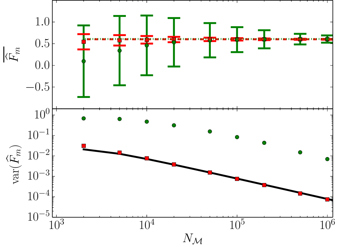
FIG. 10: Sample mean (upper panel) and variance (lower panel) of the estimators \{\widehat{F}_{\Gamma,m}\} (red square) and \{\widehat{F}_m\} (green circle) computed from the synthetic time series with \gamma = 10 . The dashed (dotted) line in the upper panel is \widehat{F}_{\Gamma} ( \widehat{F} ) computed with N data points, the black line in the lower panel is given by Eq. (16).
