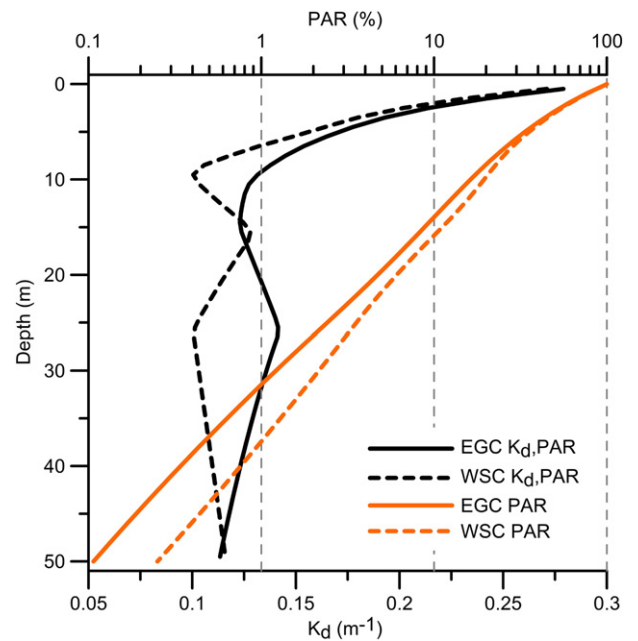
Fig. 7. Modeled vertical profiles of diffuse attenuation coefficients ( K_d ) in the EGC and WSC, and corresponding vertical profiles of PAR (logarithmic scale) in the absence of sea-ice.
