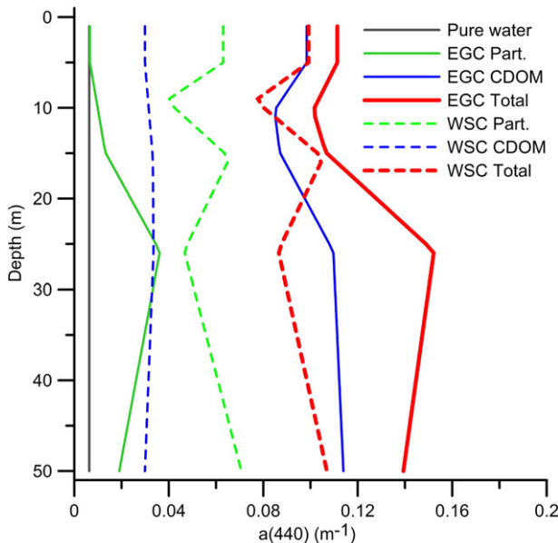
Fig. 6. Vertical profiles of absorption coefficient ( \lambda = 440 nm) by pure water, CDOM and particles used in ECOLIGHT 5.1.4 model runs.
