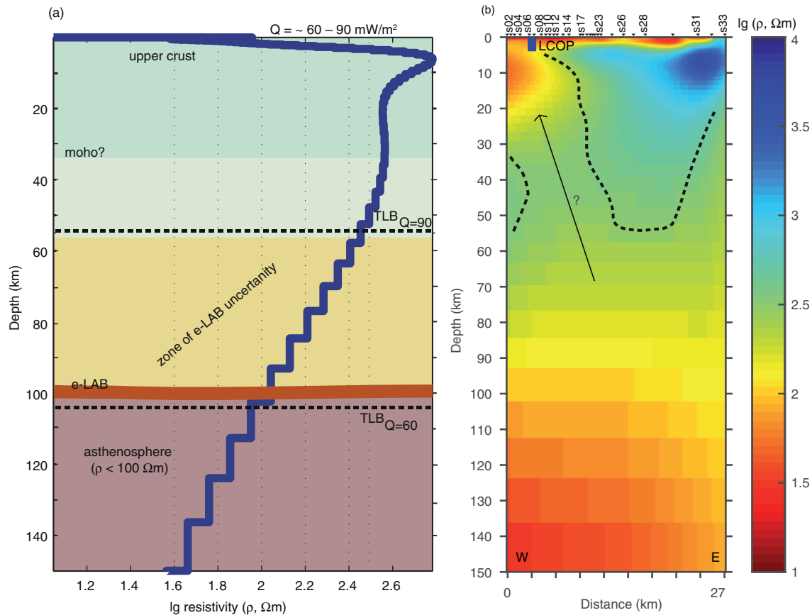
Fig. 6 Resistivity geometry from lithosphere through upper asthenosphere depth. Resistivity values are shown in \log_{10} ( \lg ) scale. (a) One-dimensional regional resistivity stratigraphy obtained from the averaged two-dimensional model shown in (b). Q is the measured surface heat-flow rate, which ranged in value from 60 to 90 \text{mW/m}^2 along the magnetotelluric (MT) profile (Pascal et al. 2011). The depth scale marked as the zone of electrical lithosphere–asthenosphere boundary (e-LAB) uncertainty falls within the calculated upper and lower thermal lithospheric base boundaries (calculated with Eqn. 2) with the specified Q . The Moho depth for Svalbard platform (ca. 30 km) is taken from Faleide et al. (2008). (b) The final two-dimensional MT model (Fig. 3) extended down to upper asthenospheric depth. The resistivity geometry marked by the arrow suggests a link between the crustal sedimentary units and the shallow convective mantle. The location of the Longyearbyen \text{CO}_2 Lab’s well park (LCOP) is marked.
