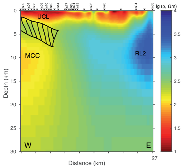
Fig. 5 A two-dimensional model example presented to show the reproducibility of the resistivity geometry seen in the final model (Fig. 3a). We obtained the model by re-running the inversion procedure using 1000- \Omega\text{m} half space as a starting model with the reduced data space Occam algorithm. This model, which is obtained after eight iterations, has the data misfit root mean square 1.06. The hatched area between the upper-crustal conductive layer (UCL) and the mid-crust conductor (MCC) indicates the section of the final model area we tested for sensitivity. The location of resistive layer 2 (RL2) is marked.
