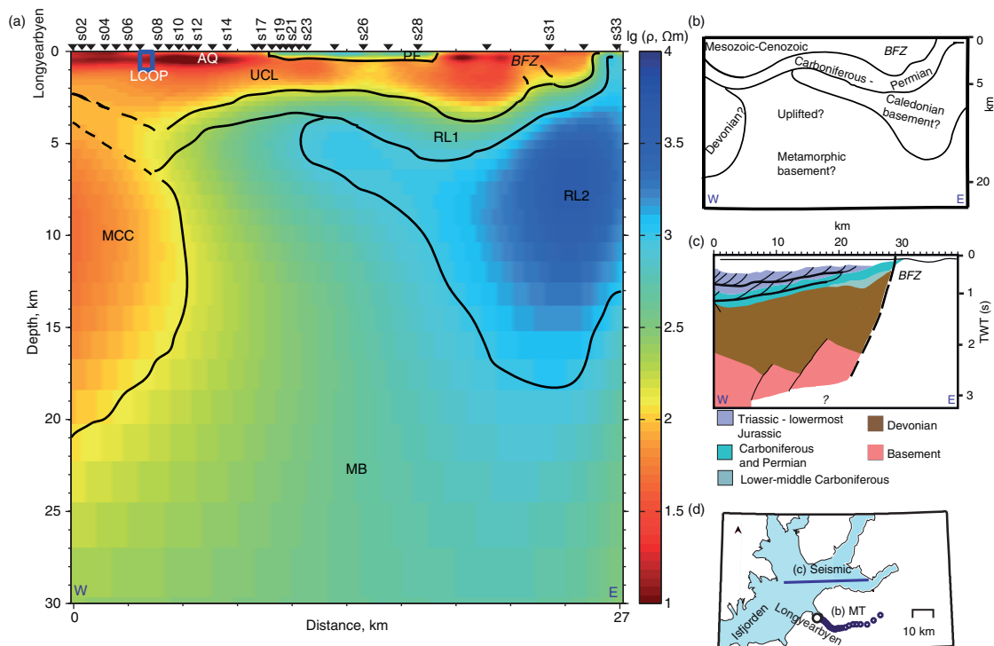
Fig. 3 (a) The final two-dimensional (2D) magnetotelluric (MT) model. The colour scale ( \lg ) is shown in \log_{10} . An error floor of 5% is assigned on the inverted data, and the inversion is started from a 100\text{-}\Omega\text{m} half-space model. The data misfit of the final model is shown in Fig. 4. (b) Geological interpretation of the MT model. (c) A schematic geological cross-section derived from a seismic section (parallel to the MT profile) in eastern Isfjorden, redrawn from Blinova et al. (2012). The y axis is given in two-way-travel time (TWT, s), where each second represents two-way-travel time (see Blinova et al. 2012). (d) The offshore seismic transect and the measured MT sites are shown in the same map to illustrate the position of the two profiles in relation to each other. Isfjorden is indicated to facilitate comparison with Fig. 1. The MT result is comparable to interpretations derived from seismic sections as in (c) and to the stratigraphic section marked by the rectangle in Fig. 1b. Geological and other features are abbreviated as follows: Longyearbyen CO 2 Lab's well park (LCOP); permafrost (PF); upper-crust conductive layer (UCL); mid-crust conductor (MCC); resistive layer 1 (RL1); resistive layer 2 (RL2); metamorphic basement (MB).
