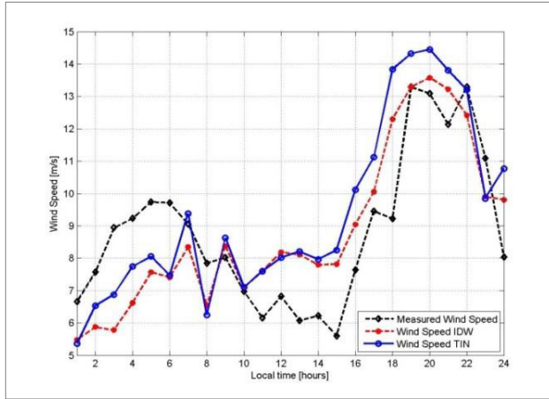
Fig. 3. Comparison of hourly wind speed (12.01.14)
