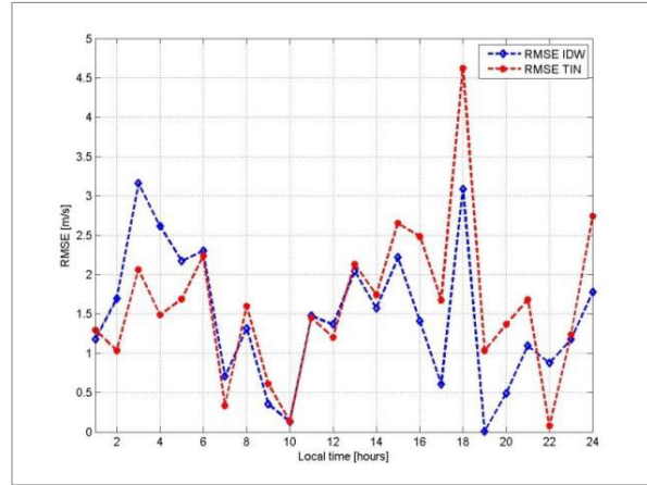
Fig. 4. Hourly root mean square error (12.01.14)
