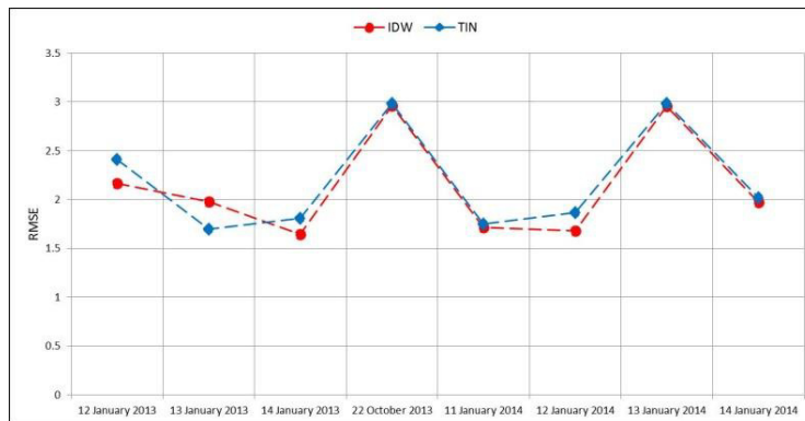
Fig. 5. Daily RMSE
