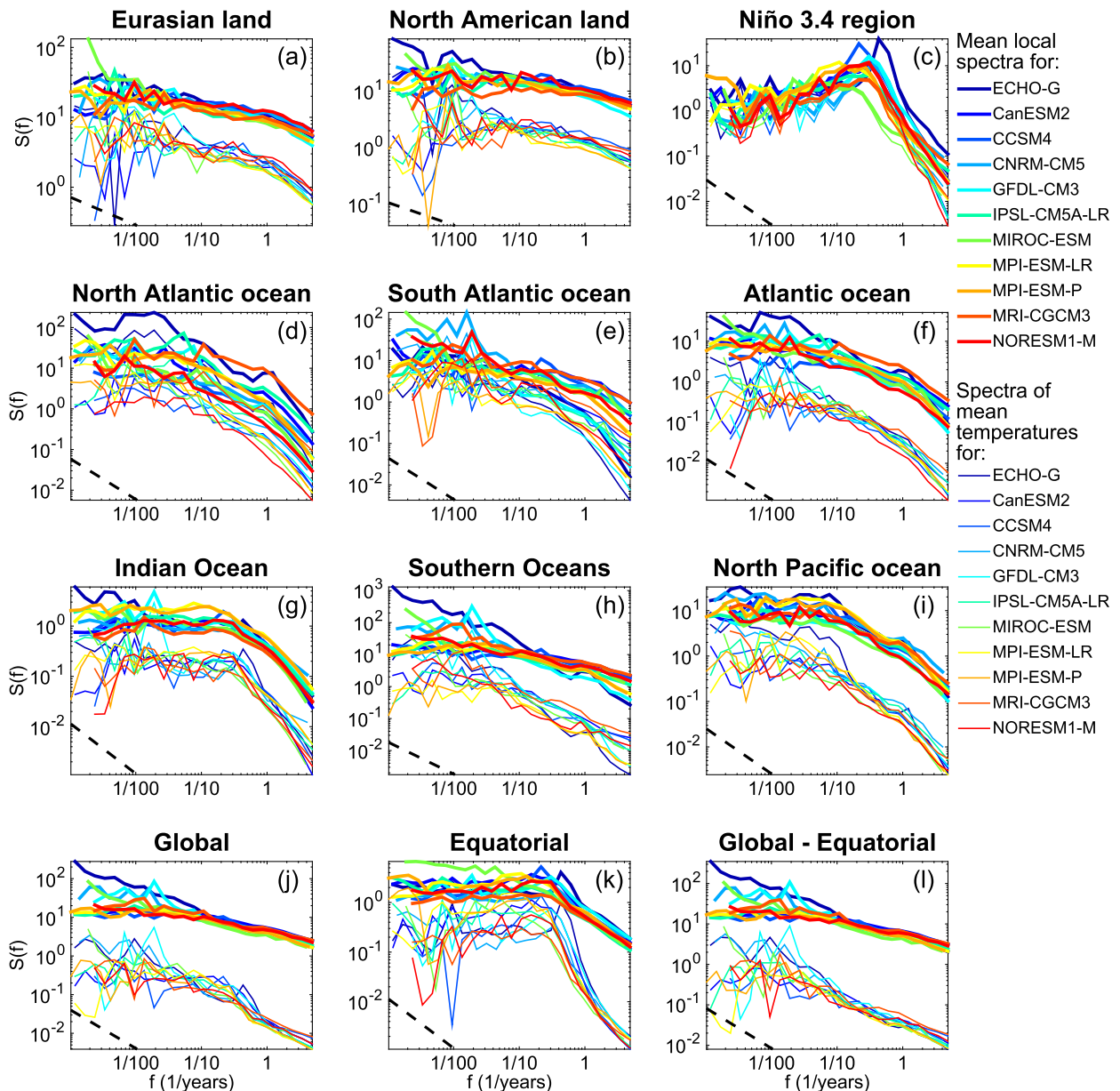
FIG. 4. The mean local spectra in several regions specified in Table 3. The thick lines are the mean spectra of the local temperatures, while the thin lines are the spectra of the mean temperature in the region. All temperatures are linearly detrended to reduce possible drifts in the climate models. The black dashed lines are reference lines with (a),(b) \beta = 0.4 for the land temperatures and (c)–(l) \beta = 1 . Note that the range of S(f) is different for each panel.
