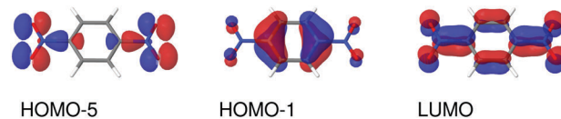
Fig. 6 Molecular orbitals involved in the electronic excitations of para -dinitrobenzene (PNB) discussed in this work. The 1B_{2g} excitation is dominated by a HOMO–5 \rightarrow LUMO transition and the 1B_{3u} excitation is dominated by a HOMO–1 \rightarrow LUMO transition. An isosurface value of 0.05 was used to make the plots.
