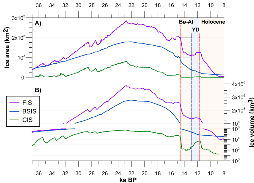
Fig. 3. Areal and volumetric changes for the three semi-independent ice sheet components of the EISC through the full Late Weichselian, extending the optimum build-up (37–19 ka BP) experiment of Patton et al. (2016). Acronyms used: CIS (Celtic ice sheet); FIS (Fennoscandian ice sheet); and BSIS (Barents Sea ice sheet). Note the log scale for CIS ice volume. Chronozones marked include the Bølling/Allerød (Bø-All) oscillation (14.6–12.9 ka BP) and Younger Dryas (YD) stadial (12.9–11.7 ka BP).
