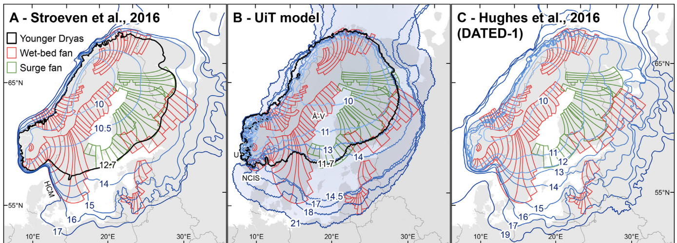
Fig. 7. Comparison of the optimum deglaciation scenario with empirically based conceptual models across Fennoscandia. Deglacial flow sets (red and green) are drawn according to landform mapping carried out by Kleman et al. (1997). A) An abridged deglaciation pattern and chronology \leq 17 ka BP according to Stroeven et al. (2016), where ice margins were predominantly reconstructed transverse to the youngest documented flow traces (e.g., eskers), marginal meltwater channels, and ice-dammed lakes. B) Retreat pattern and chronology of the optimum deglaciation scenario from this study, including the maximum Younger Dryas extent at 11.7 ka BP. C) An abridged version of the “most-credible” 1 ka timeslice reconstruction \leq 19 ka BP by Hughes et al. (2016), with limits drawn based on the distribution and ages of published numerical dates in the DATED-1 database. Acronyms used: HCM – Halland Coastal Moraines; NCIS – Norwegian Channel ice stream; U – Utsira; Å-V – Ångermanland-Västerbotten coastline. (For interpretation of the references to colour in this figure legend, the reader is referred to the web version of this article.)
