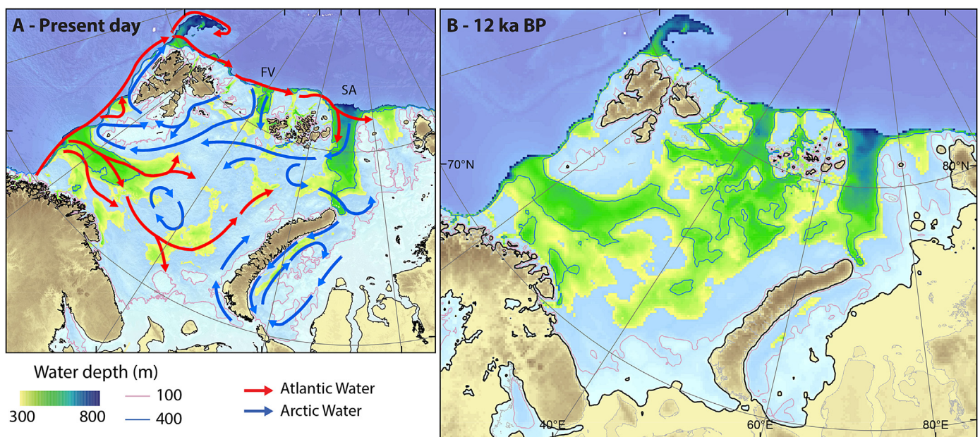
Fig. 11. A) Present day bathymetry of the Barents and Kara seas (GEMCO_2014 Grid) overlain by the main ocean currents (modified from Gammelsrød et al. (2009)). FV: Franz Victoria trough; SA: Saint Anna trough. B) Modelled bathymetry across the Barents and Kara seas at 12 ka BP, taking into account changes in relative sea level due to glacial isostatic adjustment and drops in eustatic sea level.
