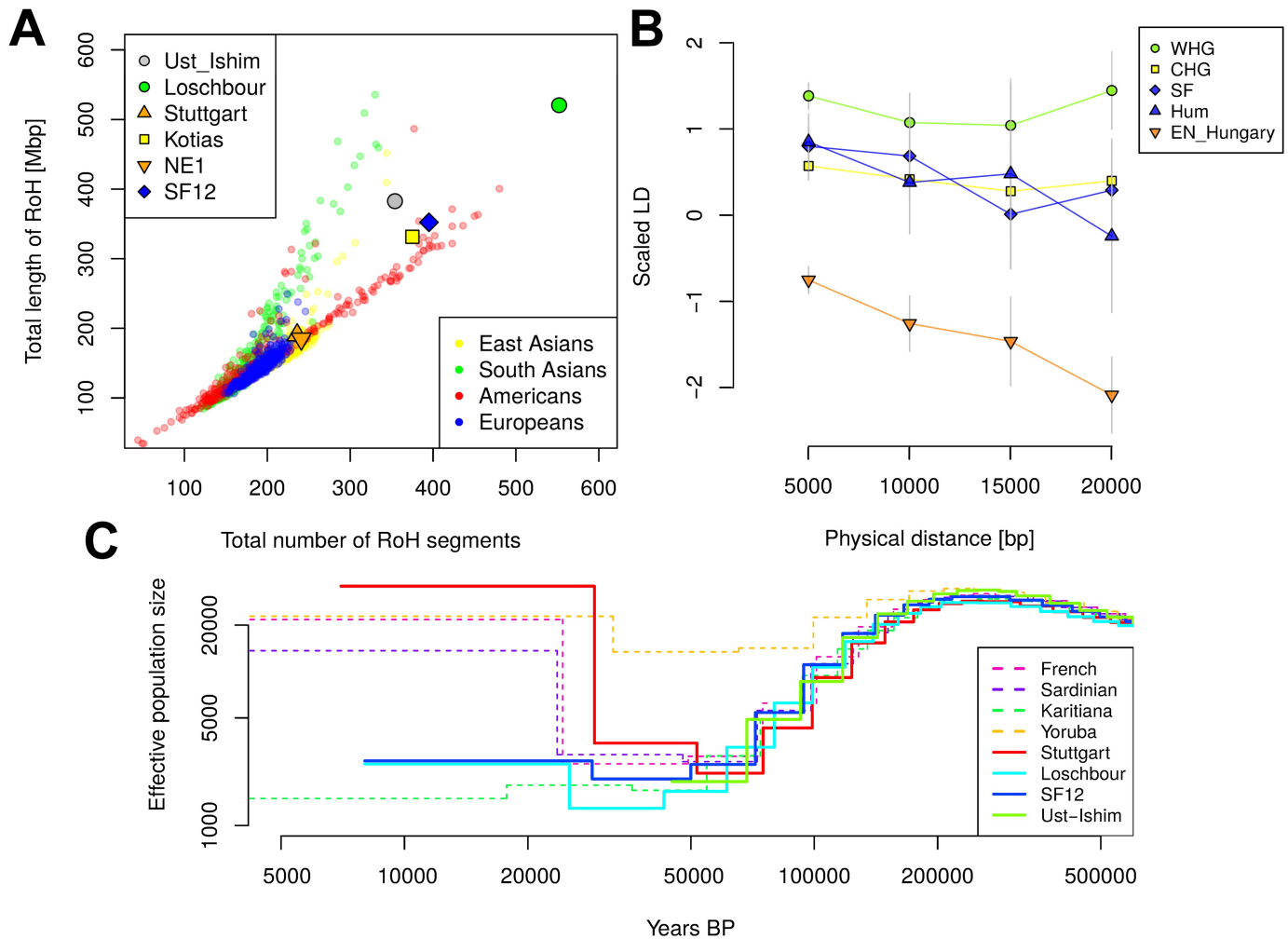
Fig 3. Genetic diversity in prehistoric Europe. (A) RoH for the six prehistoric humans that have been sequenced to >15× genome coverage, (Kotias is a hunter-gatherer from the Caucasus region [35], NE1 is an early Neolithic individual from modern-day Hungary [27], the other individuals are described in the text), compared to all modern-day non African individuals from the 1000 Genomes Project [32]. (B) LD decay for five prehistoric populations each represented by two individuals (eastern SHGs: SF [SF9 and SF12], western SHGs: Hum [Hum1 and Hum2], CHGs [35]: [Kotias and Satsurblia], WHGs [18,35] [Loschbour and Bichon], and early Neolithic Hungarians [27]: EN_Hungary [NE1 and NE6]). LD was scaled in each distance bin by using the LD for two modern populations [32] as 0 (TSI) and as 1 (PEL). LD was calculated from the covariance of derived allele frequencies of two haploid individuals per population (S7 Text). Error bars show two standard errors estimated during 100 bootstraps across SNP pairs. (C) Effective population size over time as inferred by PSMC [44] for four prehistoric humans with high genome coverage. The dashed lines show the effective population sizes for selected modern-day populations. All curves for prehistoric individuals were shifted along the x-axis according to their radiocarbon date. S4 Fig. shows 100 bootstrap replicates per individual. Data shown in this figure can be found in S1 Data. BP, before present; CHG, Caucasus hunter-gatherer; LD, linkage disequilibrium; PEL, modern-day Peruvian individual; PSMC, pairwise sequentially Markovian coalescent; RoH, runs of homozygosity; SHG, Scandinavian hunter-gatherer; TSI, modern-day Tuscan individual; WHG, western hunter-gatherer.
