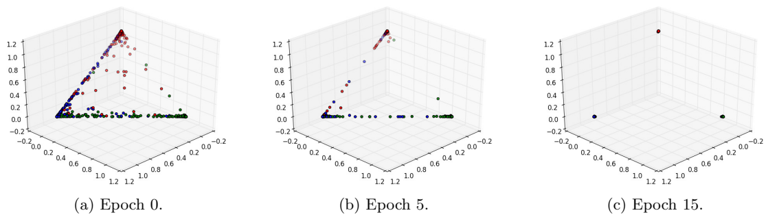
Figure 4: Illustration of DDC output space for three class MNIST training. Colors indicate class information of data points.
