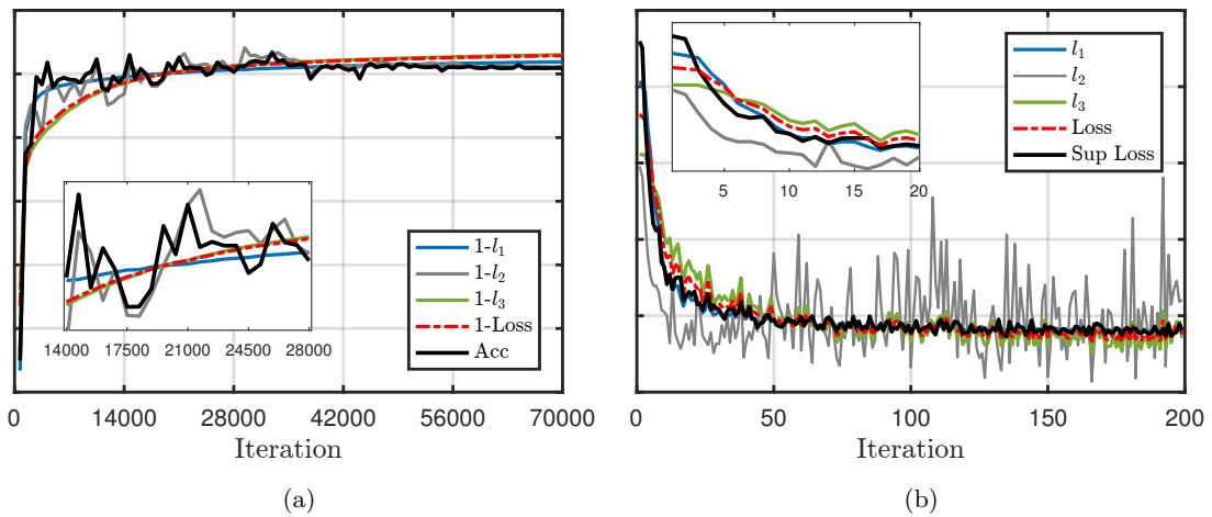
Figure 9: (a) Comparison of the supervised accuracy with the unsupervised loss function (Loss) and its three terms ( l_1 = d_{\text{hid},\alpha}, l_2 = \text{triu}(\mathbf{A}\mathbf{A}^T) , and l_3 = d_{\text{hid},m} ) during training. (b) Values of the loss function and its three terms when training the network using a supervised loss function (Sup Loss).
