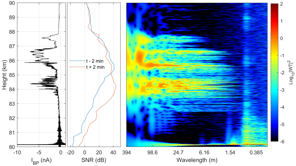
Figure 13. Comparison of DUSTY-1B bottomplate current (left panel), MAARSY 53.5 MHz radar SNR along the rocket trajectory (middle panel) and PSD from wavelet transform (right panel) – for the MXD-1B launch. The spatial scales in the right panel were converted from frequency to approximate wavelength through \lambda = 2\pi v_R/\omega , where the rocket velocity was set to that of the middle of the dust cloud; v_R = 800 \text{ ms}^{-1} . Radar data courtesy of Ralph Latteck, IAP Kühlungsborn.
