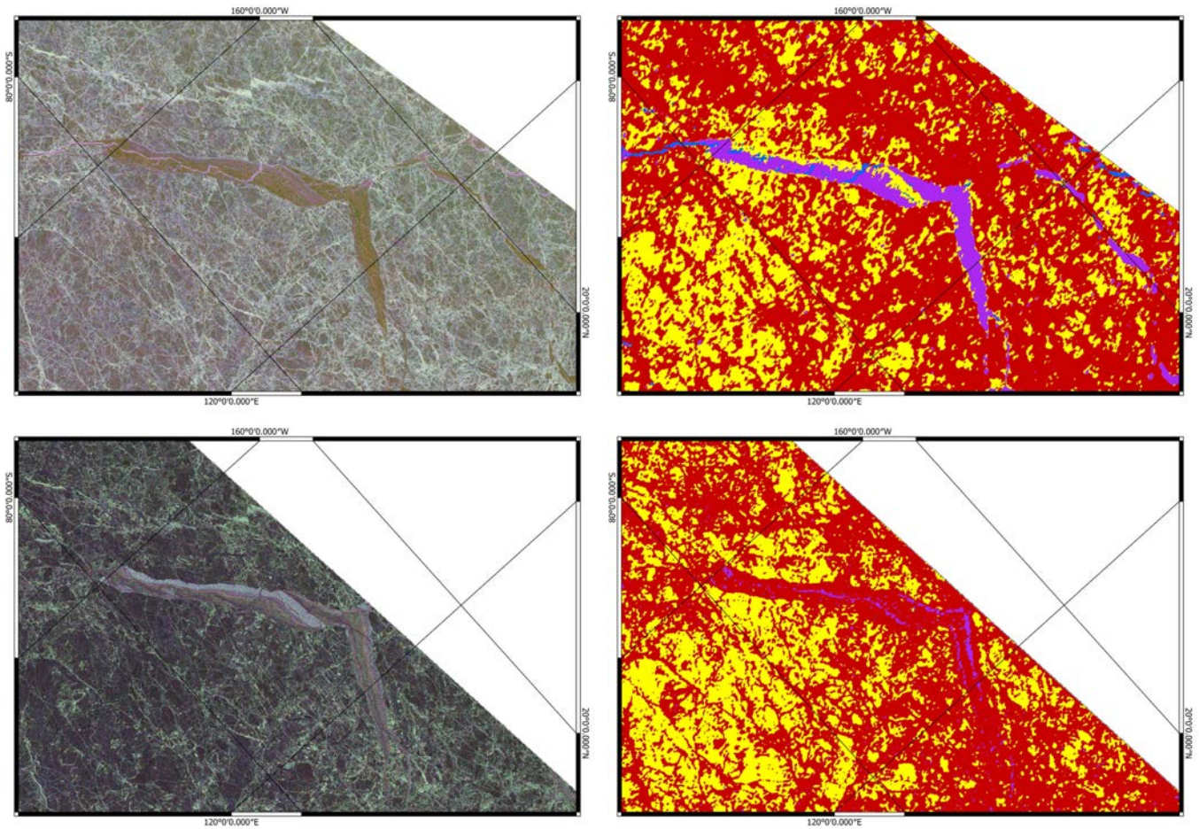
Fig. 12. (Left) Geocoded Pauli RGB composite (red: HH-VV, green: HV + VH, and blue: HH + VV) of the ALOS-2 and RS-2 acquisition on April 23, 2015. (Right) YI representation on ALOS-2 and RS-2 acquisition on April 23, 2015. Blue: open water/nilas (OW). Purple: YI. Yellow: SFYI. Red: RFYMYI.
