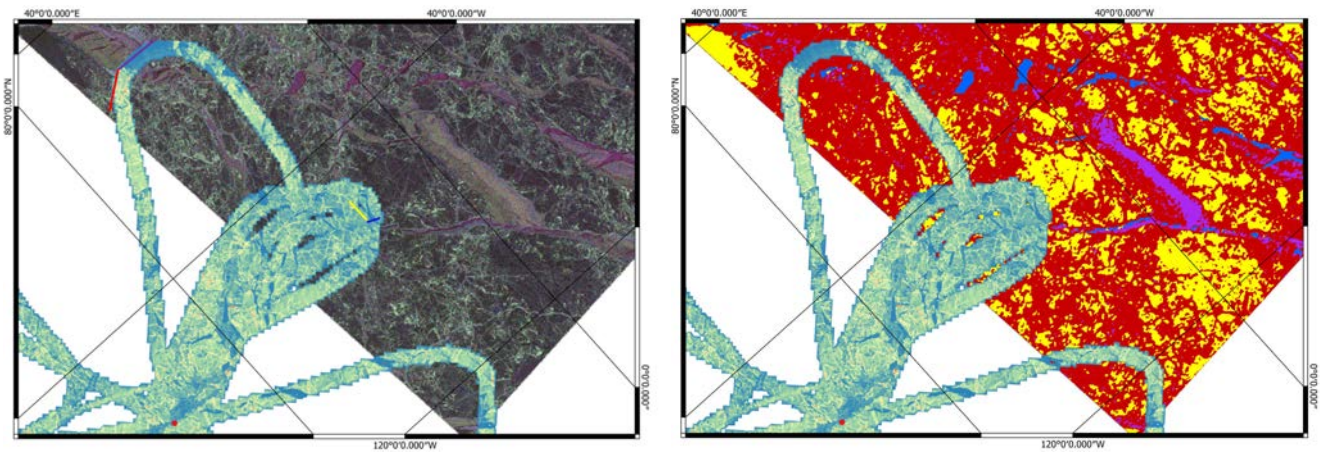
Fig. 15. (Left) ALS freeboard measurement overlaid on geocoded Pauli RGB composite (red: HH-VV, green: HV + VH, and blue: HH + VV) of the RS-2 acquisition on April 23, 2015. (Right) Ice classification on RS-2 acquisition. Blue: open water/nilas (OW). Purple: YI. Yellow: SFYI. Red: RFYMYI. ALS freeboard color scale according to Fig. 4.
