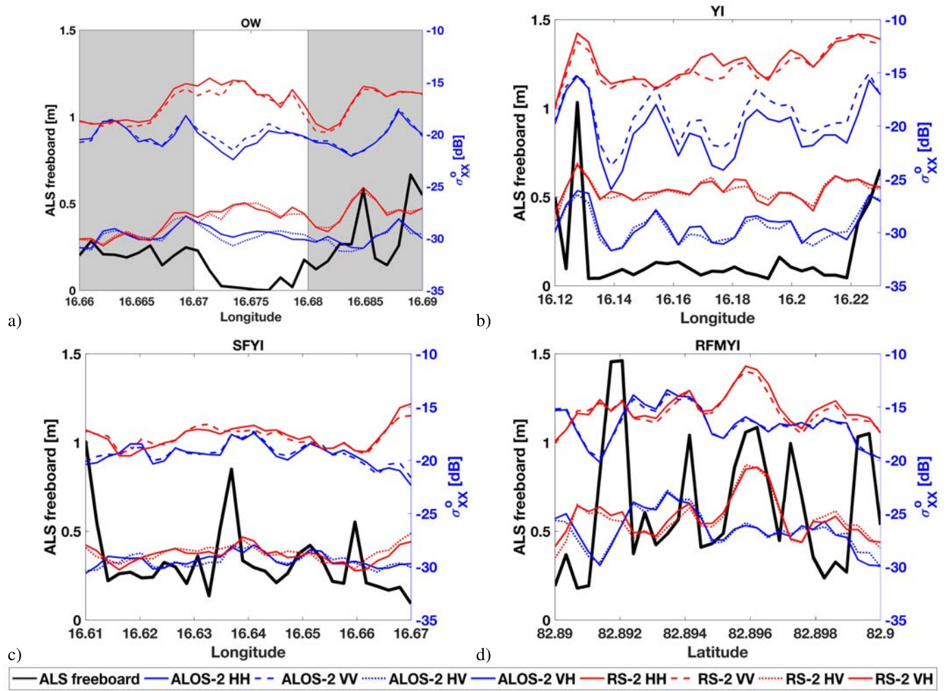
Fig. 16. Comparison of C- and L-band radar backscatter ( \sigma_{HH} , \sigma_{HV} , \sigma_{VH} , and \sigma_{VV} ) and ALS freeboard measurement over (a) open water, (b) YI, (c) SFYI, and (d) RFYMYI on April 23, 2015. Open water (blue), YI (magenta), SFYI (yellow), and RFYMYI (red) transects are indicated in Figs. 14 and 15.
