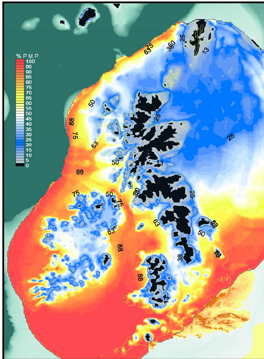
Figure 7. Cumulative time that the bed for the last (MIS 3-2) British-Irish Ice Sheet was at pressure melting point (PMP) expressed as a percentage of the total simulation time in experiment E102b2 (from Hubbard et al., 2009). Persistent frozen basal conditions given by black shading (%PMP < 2.5%). Assuming that similar basal temperatures developed beneath Early and Middle Pleistocene ice sheets, comparison with Figures 3 and 6 indicates close correlations between (i) distributions of areas with persistent cold-based ice and non-glacial landforms and (ii) areas of more frequent warm-based conditions and landscapes of glacial roughening and streamlining.
