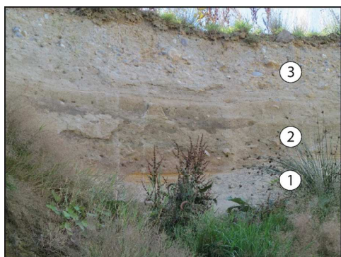
Figure 23 Savock Quarry in 2014. Section ca. 5 m high: 1. Middle Pleistocene sand and gravel channel fill. 2. Brown, possibly weathered till correlated with the MIS 6 Rottenhill Till Formation at Toddlehills, Leys and Kirkhill. 3. Upper clast-rich till correlated with the MIS 3-2 Hythie Till.
