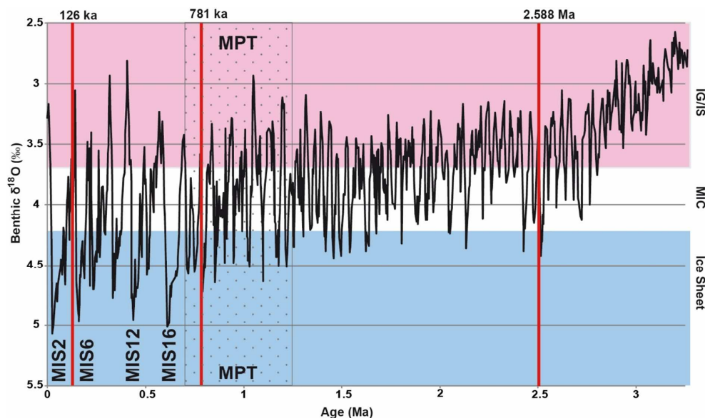
Figure 1 The \delta^{18}\text{O} record for benthic foraminifera from marine core DSDP 607 (Ruddiman et al. , 1989) interpreted as a proxy for glacier extent in Scotland. The cut-off value of >3.7\text{‰} \delta^{18}\text{O} indicates when conditions were equivalent to the Younger Dryas event (Small & Fabel, 2016) when mountain ice caps, valley and corrie glaciers formed in Scotland (Clapperton 1997). The cut off value of >4.2\text{‰} \delta^{18}\text{O} is that at 37.5 ka in DSDP 607, a time when the last ice sheet started to build up in Scotland (Hubbard et al. 2009). IG - interglacial; IS - interstadial; MIC - mountain ice cap; MPT - Mid-Pleistocene Transition. Marine isotope stages (MIS) marked are equivalent to the following British and NW European stages: MIS 16 (676-621 ka; Happisburgh-Donian), MIS 12 (478-424 Ma; Anglian-Elsterian), MIS 6 (186-130 ka) (Wolstonian-Saalian) and 2 (29-14 ka; Late Devensian-Late Weichselian).
