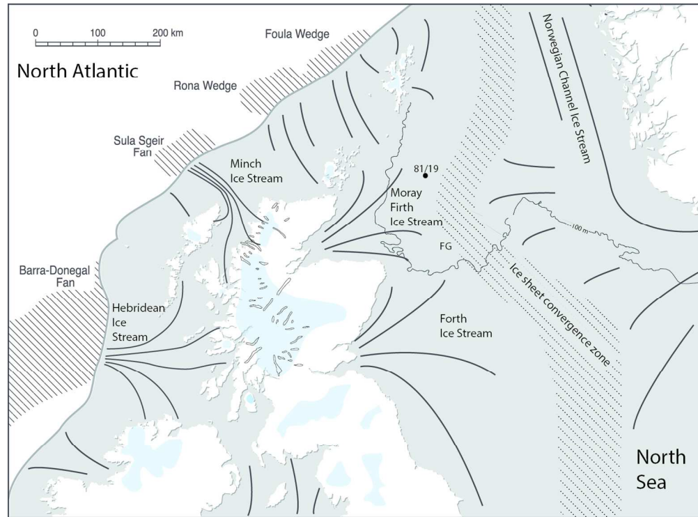
Figure 2. Main features of the Pleistocene glacialiation of Scotland. Major and minor centres of ice sheet growth are shaded in blue. Note the ribbon lakes in the western Highlands and the associated rock basins of the inner sea lochs of the west coast that together define a belt of glacial over-deepening beneath former mountain ice caps. IS ice stream. FG Fladen Ground. IS Ice Stream.
