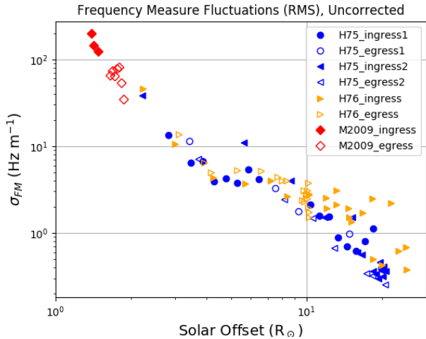
Figure 4. Composite of the frequency measure fluctuations, \sigma_{FM} . The MESSENGER data were obtained in a one-way radio configuration. The 2-way HELIOS data shown here were taken directly from JPL technical reports, normalized to radio wavelength, but not yet corrected for correlated 2-way propagation inhomogeneities and the difference in effective frequency band.
