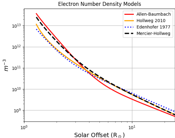
Figure 7. Electron number density models. Our composite model, combining the fit from Mercier and Chambe (2014) with the second term from Hollweg et al. (2010) is shown with a dashed line. For comparison, the Allen-Baumbach, Hollweg and Edenhofer models are given.
