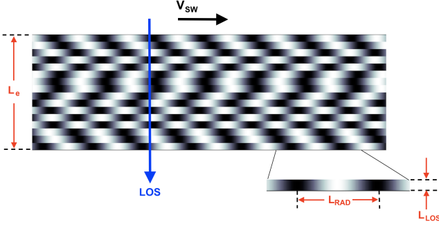
Figure 5. The simplified scheme of oscillating density fluctuations aligned parallel to the magnetic field, in a series of stacked flux tubes. Each horizontal strip contains plasma density oscillations, illustrated by brightness variations. L_{RAD} is the horizontal length scale for convected quasi-static density disturbances. The vertical scale L_{LOS} corresponds to width of a flux tube. The bulk plasma frame outflow speed is V_{sw} . Individual flux tube density fluctuations combine with random-walk statistics to yield the RMS fluctuation for the effective LOS, L_e .
