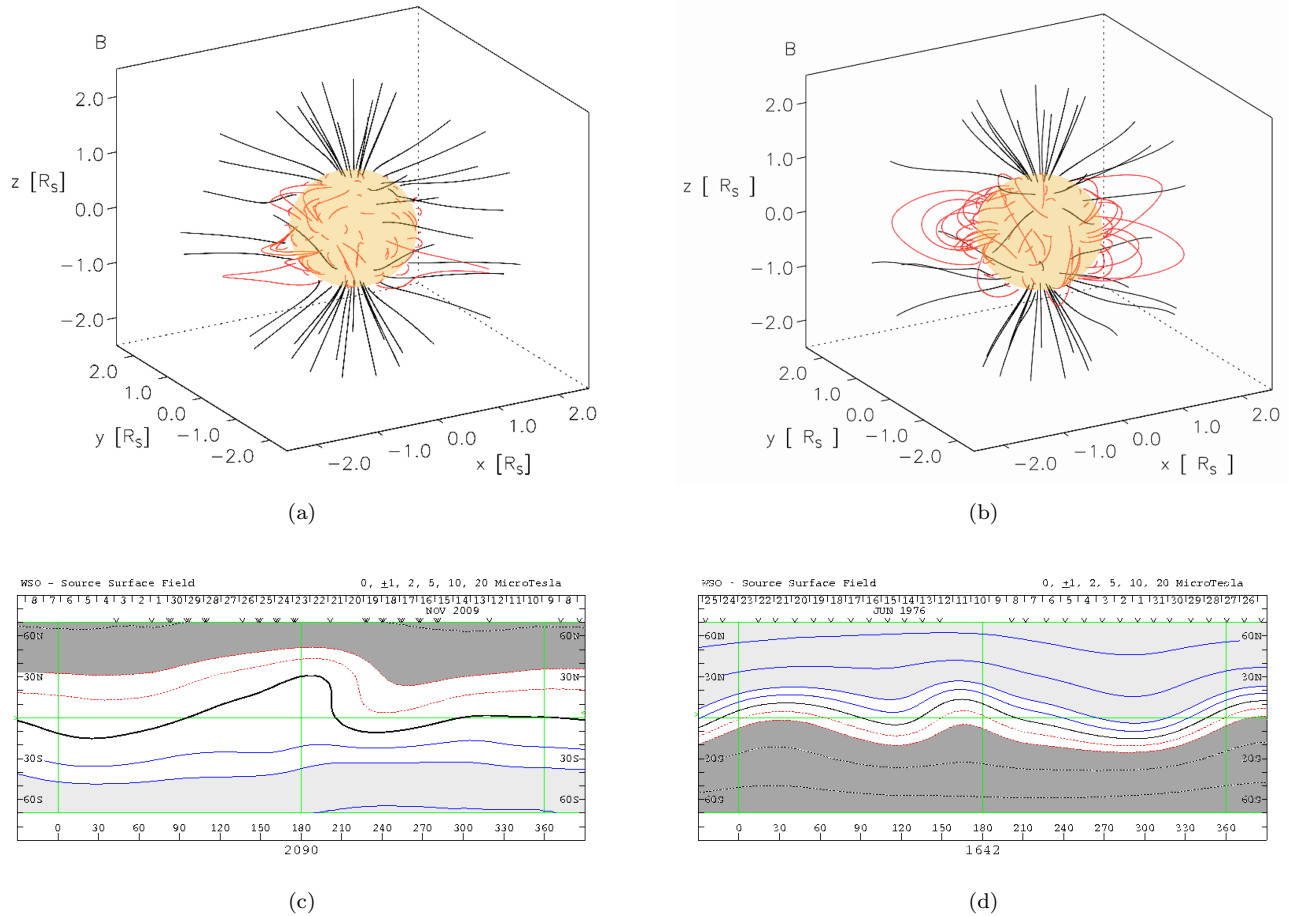
Figure 1. Magnetic field modeling from solar surface to 2.5R_{\odot} from the Community Coordinated Modeling Center. (a) CR 2090, MESSENGER egress data 2009, (b) CR 1642, corresponding to part of the HELIOS 2 data 1976. Potential field source surface magnetic maps ( 2.5R_{\odot} ) for the Wilcox Solar Observatory: (c) MESSENGER CR 2090 (d) HELIOS CR 1642.
