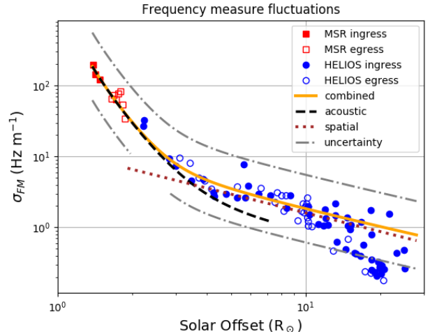
Figure 9. The composite MESSENGER-HELIOS frequency measure observations, shown with results of the frequency fluctuation model of combined component variances (equation 30). Acoustic wave contributions with \epsilon_{BL} = 0.017 are shown with the dashed line, while the convected spatial density variations with L_{RAD}=12000 km are shown the dotted line. Uncertainty limits for the model are indicated with the dot-dashed lines.
