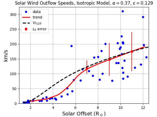
Figure 10. Solar wind velocity results using the isotropic turbulence equation (solid line - trend; dots - individual data points). For comparison, the V_{flux} (mass continuity) curve is shown as a dashed line. The illustrated error limits were based only on the uncertainty in the outer scale of turbulence.
