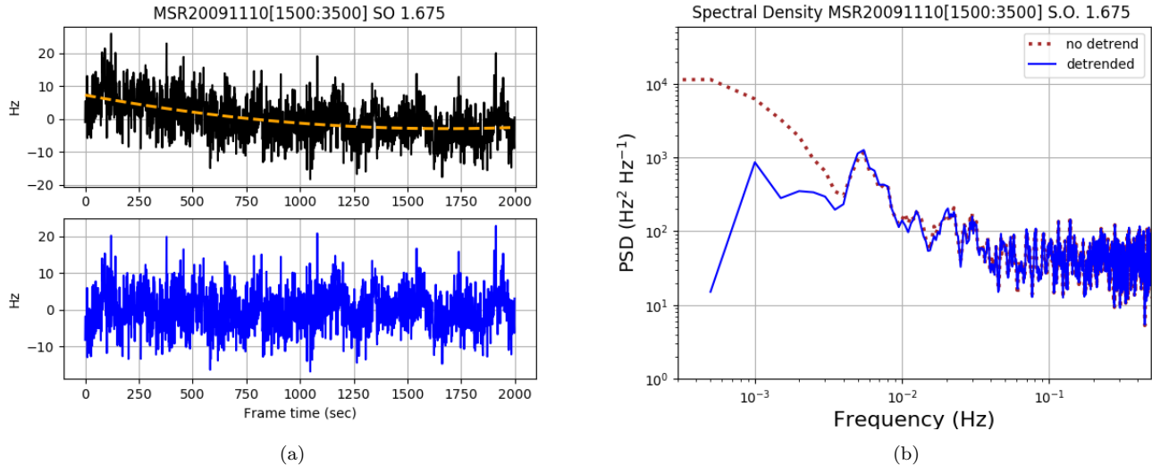
Figure 3. Left: Time series of zero-centered frequency data. Upper panel shows the frequency fluctuation (FF) time series for a 2000-second analysis frame, at SO 1.675 R_{\odot} . The dashed line is the second order polynomial used to remove the slow trend attributed to the Doppler shift of spacecraft motion. The lower panel shows the FF time series after the detrend procedure was applied. Right: Power spectral density (PSD) of the FF analysis segment. The detrend procedure affects mostly low-frequency spectral power, as shown with the dotted line. In this sample, enhancement of spectral power over 5-7 mHz relative to the background spectrum is noted.
