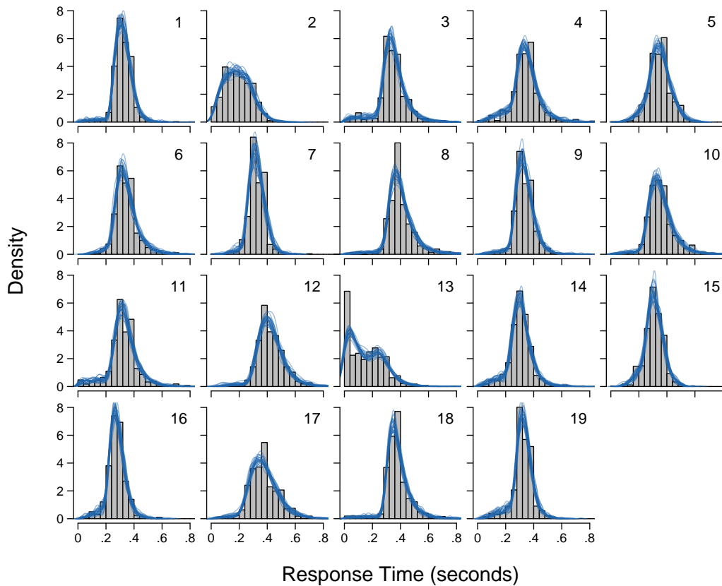
Figure 5. Individual participant response time distributions (gray histograms) with overlaid posterior predictive distribution of the rhythmic race model (blue density curves) from Experiment 1. The posterior predictive distribution shows a sample of 25 predicted distributions of response times that were generated from 25 independent random samples of parameter values from the posterior distribution of the parameters.
