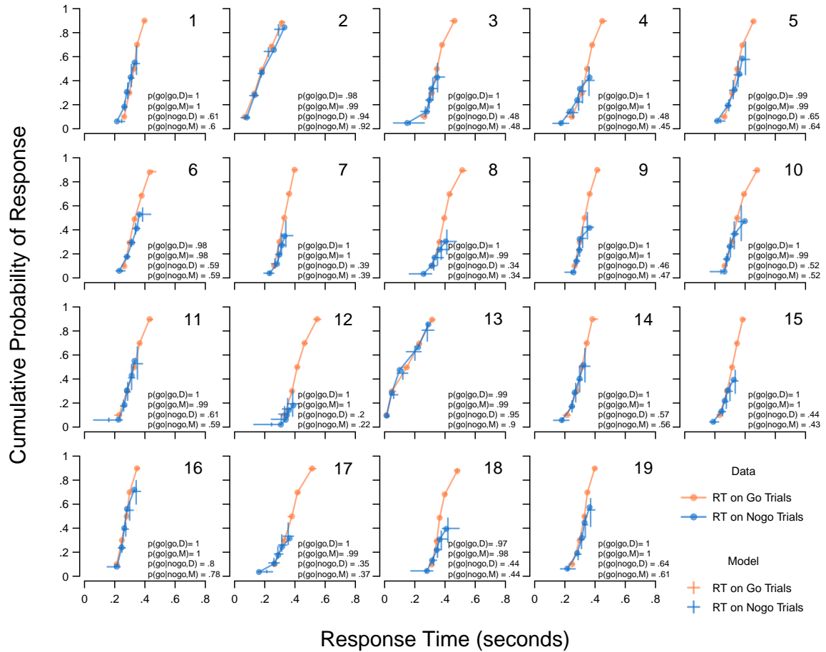
Figure 6. Defective cumulative distribution functions showing data and the posterior predictive distribution of the rhythmic race model for individual participant data from Experiment 1. Points along the x -axes show the 10 th , 30 th , 50 th (i.e., median), 70 th and 90 th percentiles of the RT distributions for go (correct; orange) and nogo (error; blue) responses. Points along the y -axes show the cumulative probability of a response. Data are shown as circular symbols connected with lines. The posterior predictive distribution for the 5 percentiles of each RT distribution is shown as crosses, where the center (respectively, horizontal and vertical arms) of the cross indicates the expectation (respectively, 95% credible intervals). Where the crosses cannot be seen, the 95% credible interval is smaller than the overlaid data symbol. The lower right of each panel displays the proportion of go (i.e., observed) responses on go and nogo trials observed in data for each participant, p(\text{go}|\text{go},D) and p(\text{go}|\text{nogo},D) , respectively, and the same quantities as predicted by the model, p(\text{go}|\text{go},M) and p(\text{go}|\text{nogo},M) .
