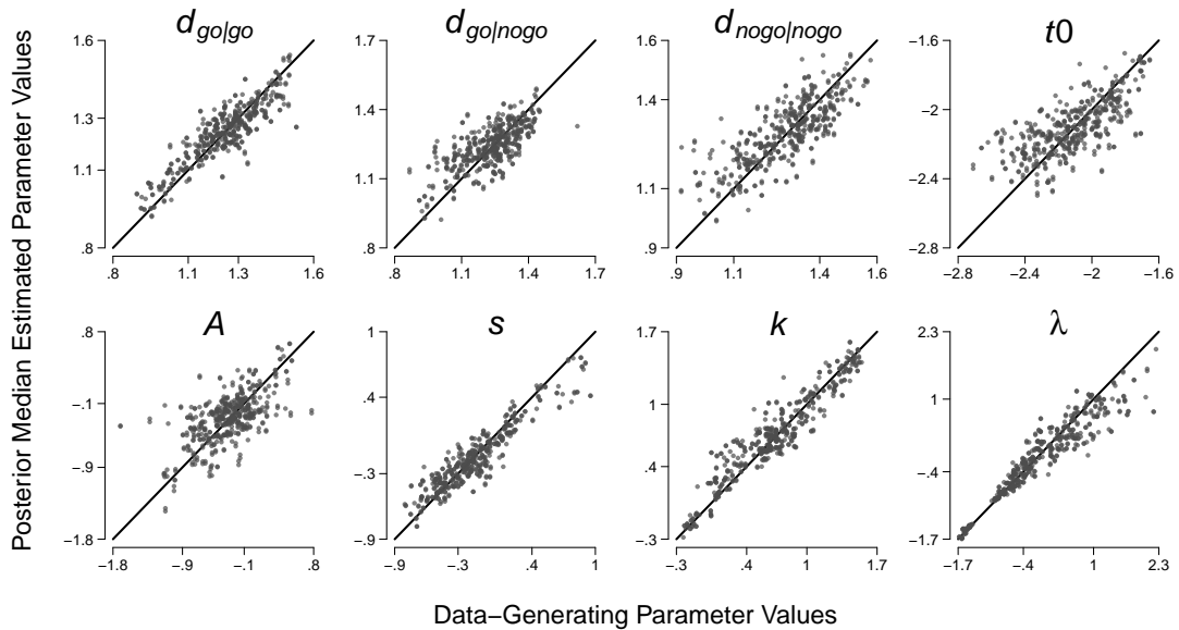
Figure E1. Parameter recovery for the RRM. Model parameters are shown in separate panels, data-generating parameter values are shown along the x -axes, and the median of the estimated posterior distributions are shown on the y -axes. Perfect parameter recovery is indicated along the diagonal. Parameters are shown in the transformed space in which they were estimated (logit scaling for A , log scaling for all other parameters; Appendix D).
