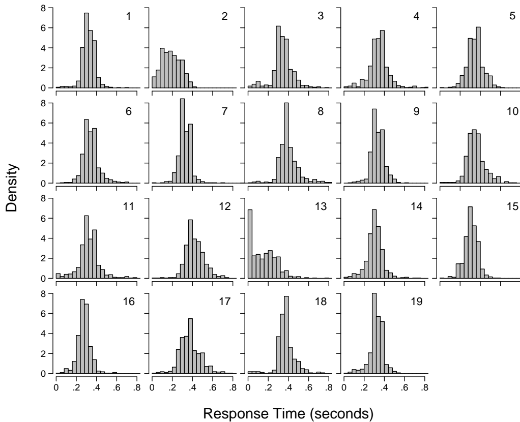
Figure 2. Individual participant response time distributions from Experiment 1.
