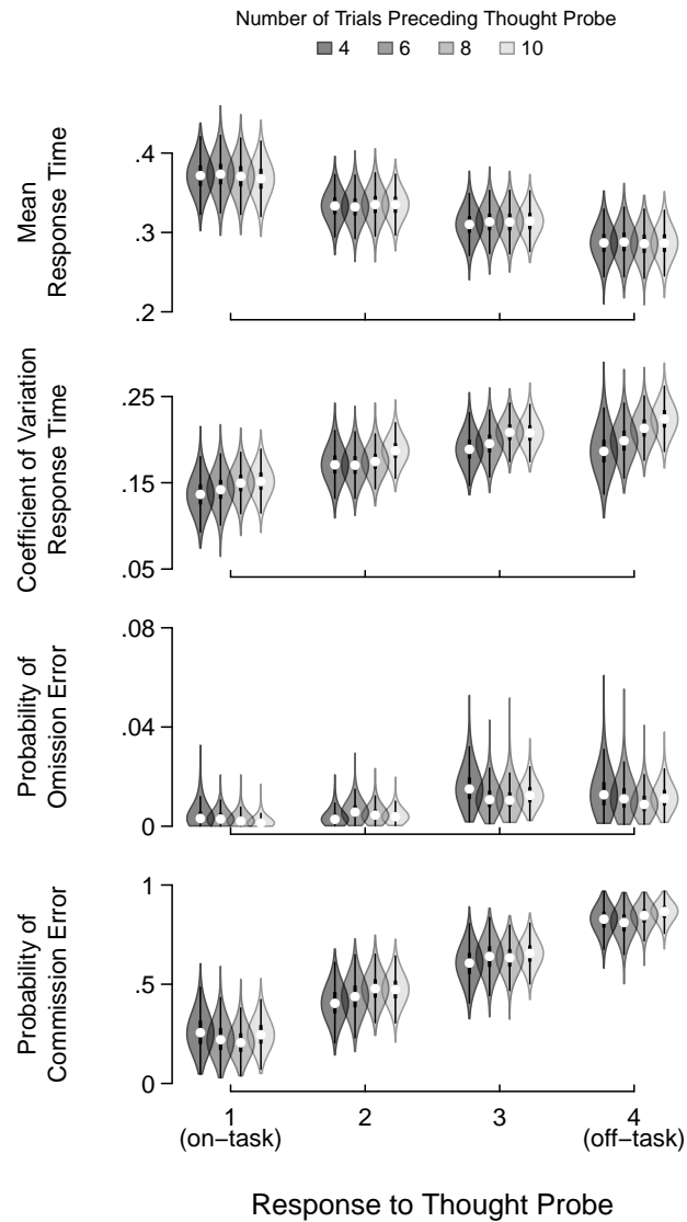
Figure 1. Posterior distributions of the group-level effects from the Bayesian data analysis of the 4 outcome measures (shown in rows) in Experiment 1. The estimated outcome measures ( y -axes) are shown as a function of each probe response ( x -axes). The window size, the number of trials preceding each thought probe response over which the outcome measure was calculated, is shown with the shade of the ‘violin’ plots. The violin plots represent the posterior distribution of the estimated parameters, where each ‘violin’ combines a boxplot and a kernel density estimate. The boxplot component is indicated with the white circular symbol (median), the interquartile range (heavy vertical line), and 1.5x interquartile range as an indicator of the range of the posterior distribution (thin vertical line). The ‘violin’-like shape of each distribution is obtained through a smoothed density estimate of the posterior distribution, rotated vertically, and plotted on both sides of the box plot to create a symmetric figure. The width of the violin is proportional to the number of samples that fall in that part of the posterior distribution.
