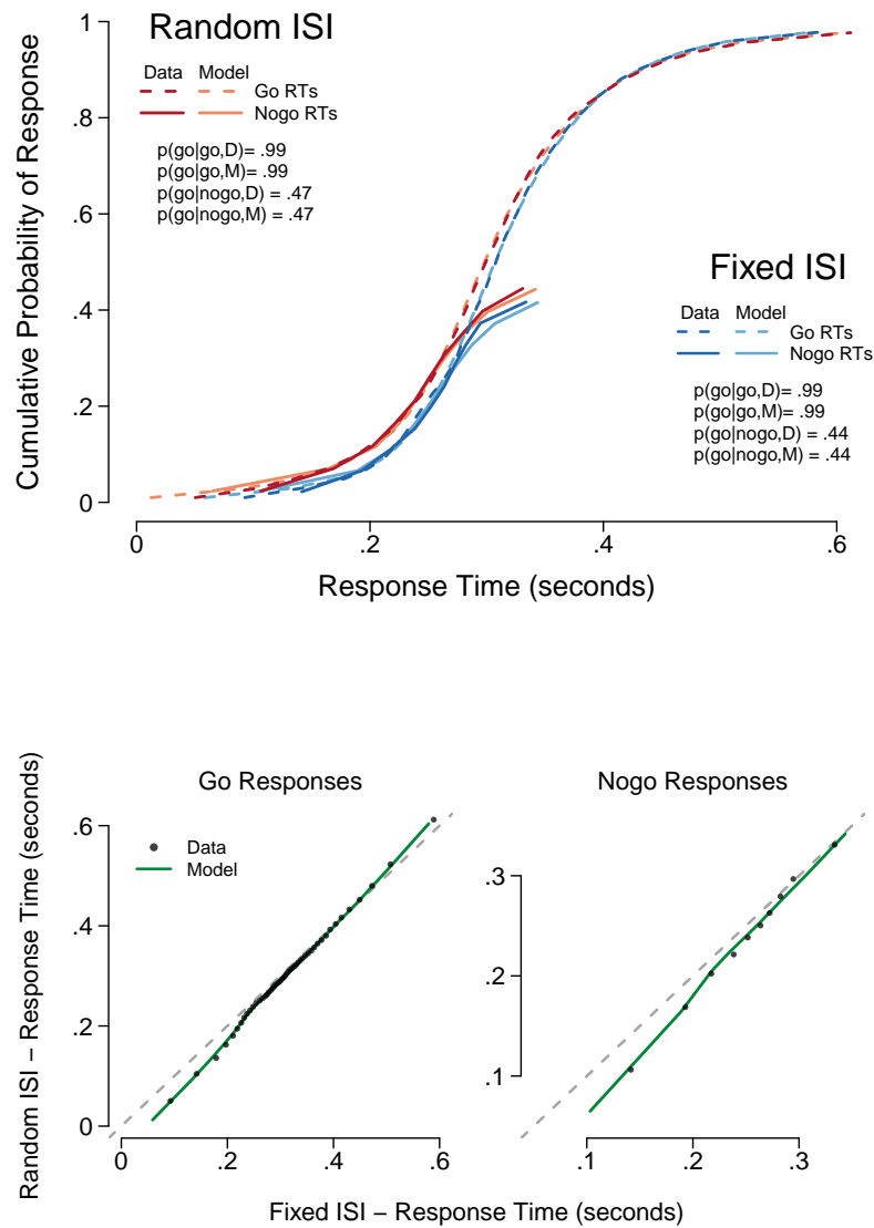
Figure 9. Defective CDFs showing group-averaged data with overlaid group-averaged posterior predictive distribution of the rhythmic race model from Experiment 2 (upper panel), and quantile-quantile plots showing the difference in RT distributions for go and nogo responses between the random and fixed ISI conditions (lower panels). Upper panel: Go and nogo RTs are shown in dashed and solid lines, respectively. Quantile averaged data and posterior predictive distribution are shown in red shades (random ISI) and blue shades (fixed ISI), respectively. The mean proportion of go (i.e., observed) responses on go and nogo trials, p(\text{go}|\text{go},D) and p(\text{go}|\text{nogo},D) , respectively, and the same quantities as predicted by the model, p(\text{go}|\text{go},M) and p(\text{go}|\text{nogo},M) , are shown for the random and fixed ISI conditions. Lower panels: Percentiles of the RT distributions from the random and fixed ISI conditions are displayed as a quantile-quantile plot for go responses (left) and nogo responses (right). Data and posterior predictive distribution are shown in black dots and green lines, respectively.
