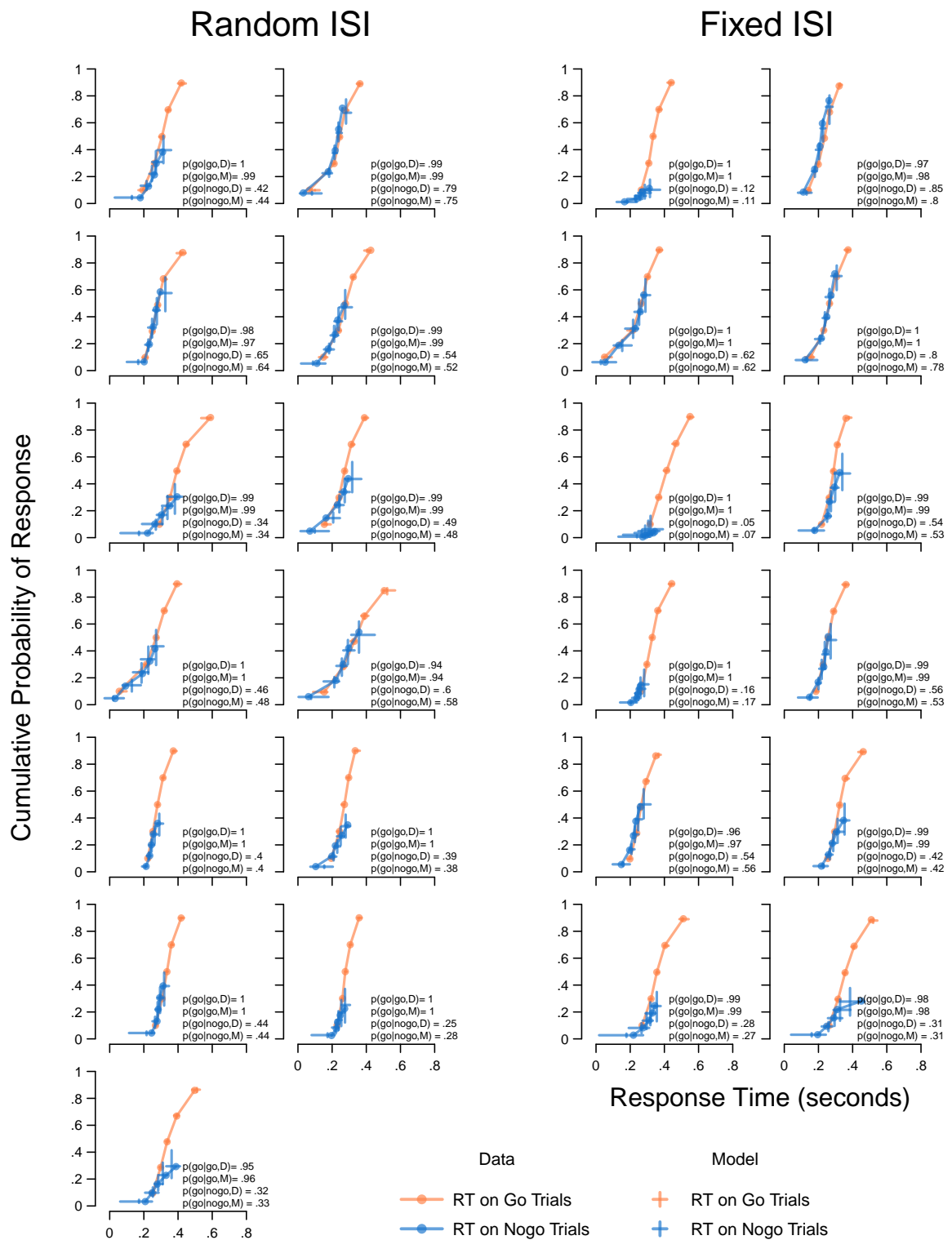
Figure 8. Defective CDFs showing data and the posterior predictive distribution of the rhythmic race model for individual participant data from Experiment 2. All details are as described in Figure 6 with the exception that data and posterior predictive distributions for the random and fixed ISI conditions are shown in the left and right columns, respectively.
