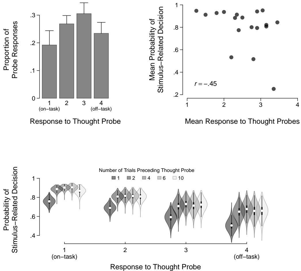
Figure 7. Analysis of thought probe data. The barplot (upper left) shows the distribution of thought probe responses, averaged across participants. The scatter plot (upper right) shows the across-participant relationship between the probability of a stimulus-related decision as predicted by the RRM ( p(\text{decision}) ; y -axis) and self-reported task-unrelated thoughts ( x -axis), where each point represents each participant’s mean across both measures. The violin plot (lower row) shows the posterior distribution of the group-level effect from the Bayesian data analysis of p(\text{decision}) , in the same format as Figure 1. The estimated probability of a stimulus-related decision ( y -axis) is shown as a function of each probe response ( x -axis). The window size, the number of trials preceding each thought probe response over which p(\text{decision}) was averaged, is shown with the shade of the violin plots. All other details are as described in Figure 1.
