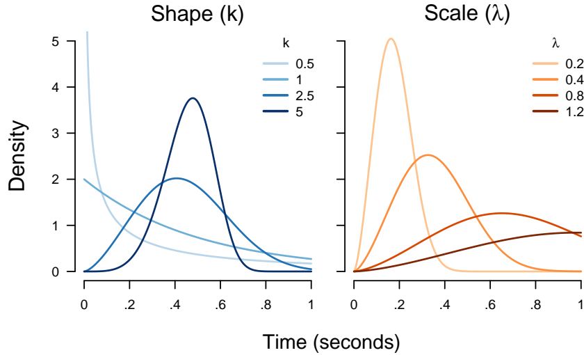
Figure 4. Illustration of various Weibull distributions. The left panel plots a family of Weibull distributions across a range of shape parameters ( k ) with a fixed value of the scale parameter ( \lambda = .5 ). The right panel plots a family of Weibull distributions across a range of scale parameters ( \lambda ) with a fixed value of the shape parameter ( k = 2.5 ).
