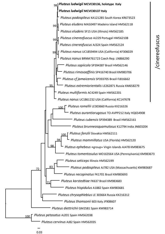
The ITS phylogenetic tree was inferred using the Maximum likelihood (ML) method based on the GTR+G model in RAXML v. 8.2.1. Only bootstrap values ≥ 70 % are indicated on the nodes (1 000 bootstraps).
