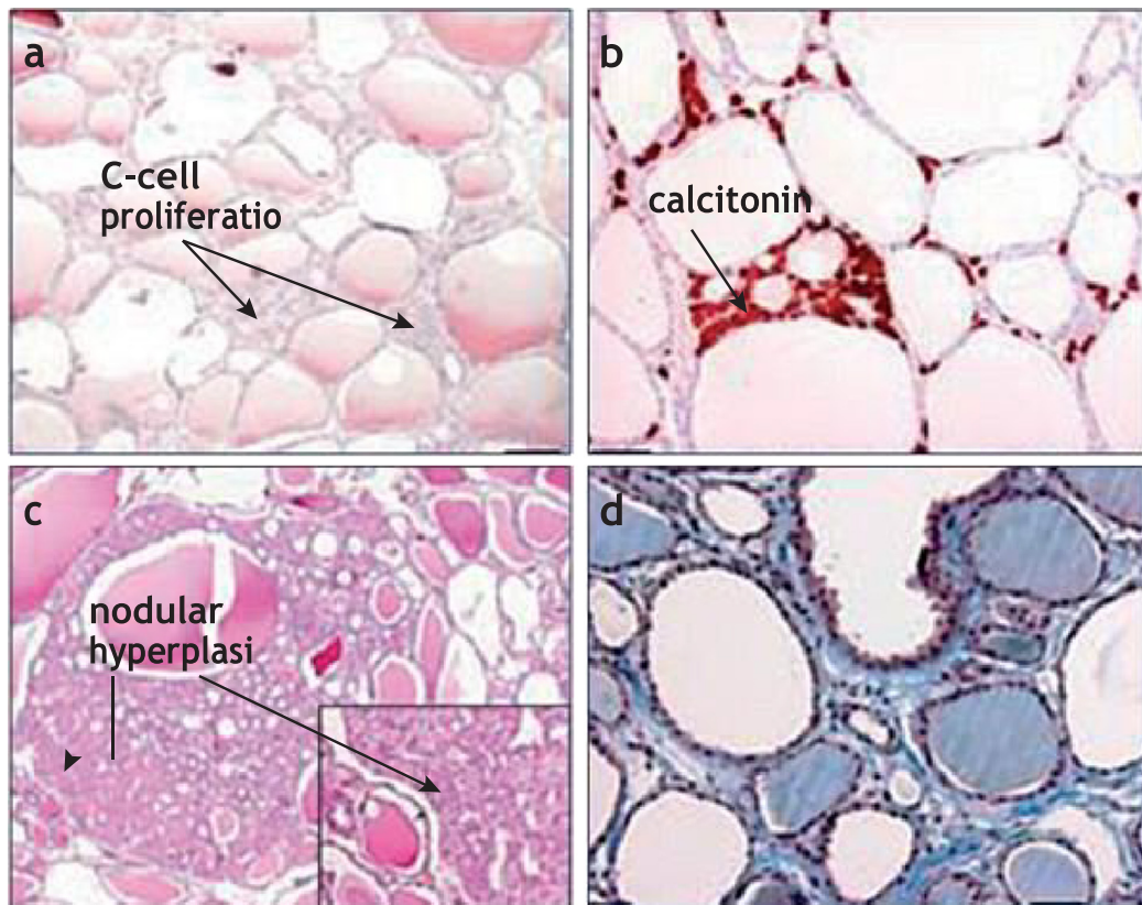
Fig. 4. Thyroid lesions in East Greenland polar bears sampled during 1999–2009. (a) C-cell proliferations. (b) calcitonin colouring. (c) nodular hyperplasia. (d) interstitial fibrosis. (Modified from Sonne et al., 2011).
