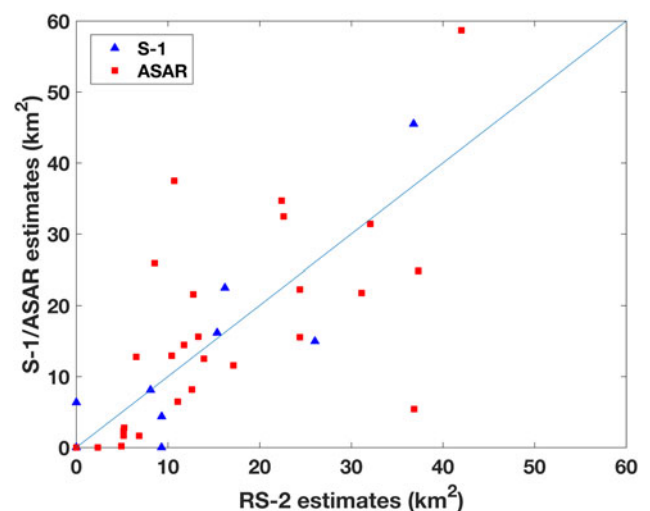
Fig. 3. Comparison between fjord ice area estimates in ASAR/RS-2 and RS-2/S-1.
