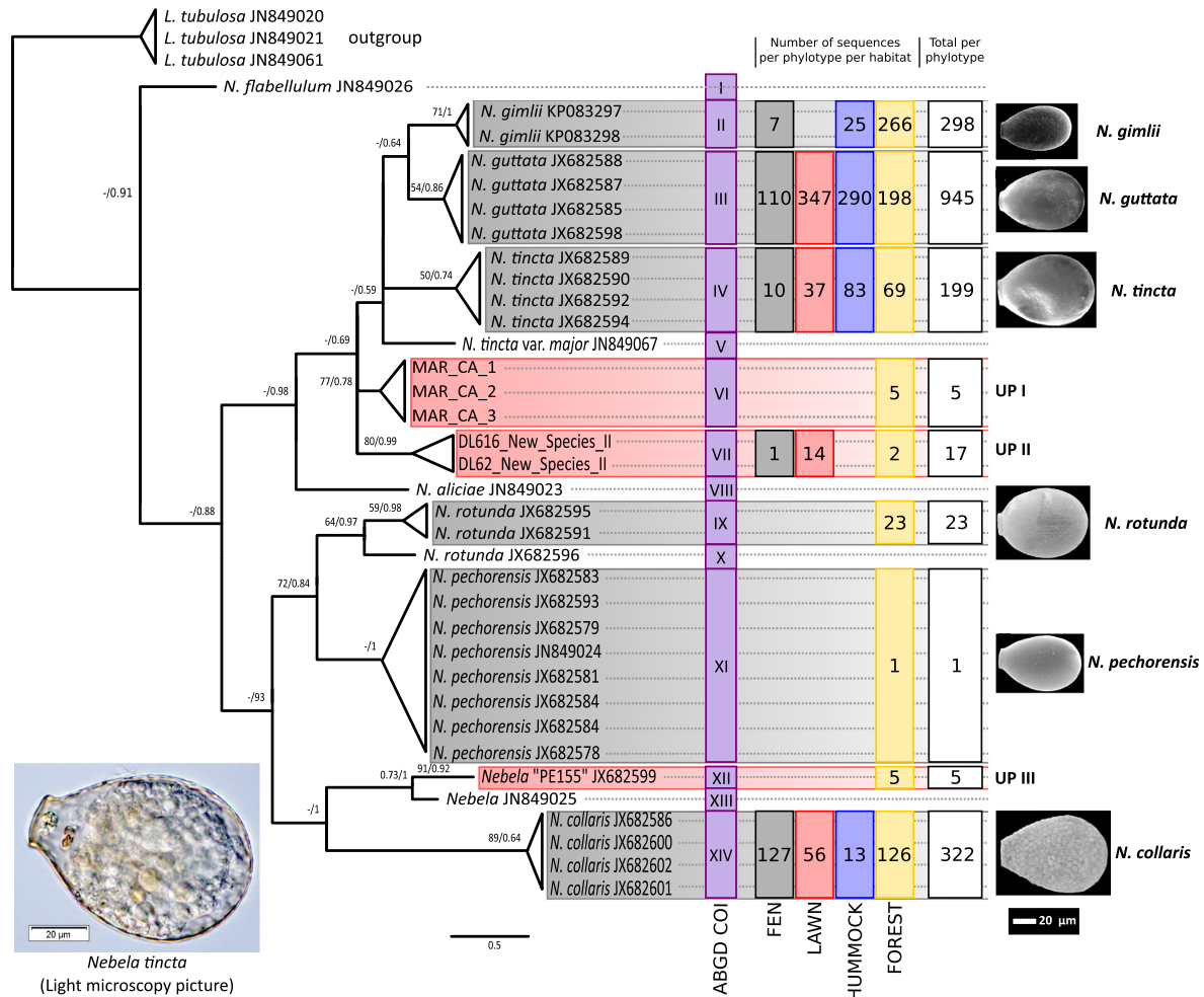
FIG. 1. Bayesian Markov Chain Monte Carlo consensus tree of 32 single cells of Nebela collaris s.l. mitochondrial cytochrome oxidase, subunit I (COI) sequences from two peatlands in the Swiss Jura Mountains and 1,028 environmental sequences, plus three sequences of Longinebela tubulosa as outgroup. The numbers along the branches represent, respectively, bootstraps obtained by maximum likelihood method and posterior probabilities as calculated with Bayesian analyses. Only values above 50/0.50 are shown. Sample colors indicate the five different habitats within peatlands (red = lawn, yellow = forest, blue = hummock, black = fen).
