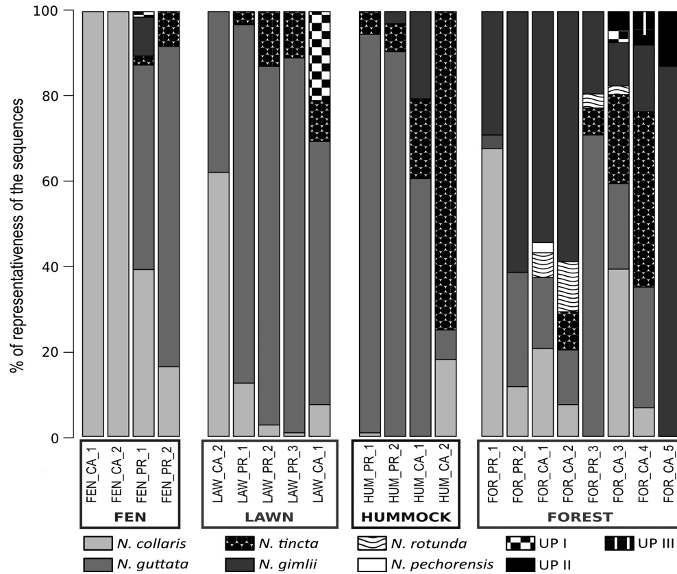
FIG. 2. Community profiles of testate amoebae from the Nebela collaris complex s.l. extracted from Sphagnum samples from two peatlands in the Swiss Jura Mountains. Each barplot represents the relative ratio of the clone sequences corrected by the cell biovolume (Kosakyan et al. 2015). The phylotypes that are not related to any known species are represented by “UP” (Unknown Phylotype).
