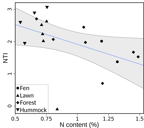
FIG. 4. Nearest Taxon Index (NTI) values from Nebela collaris s.l. communities extracted from Sphagnum samples collected from two peatlands in the Swiss Jura Mountains in function of Sphagnum Nitrogen content (%). The line shows the linear regression ( P = 0.004 ) and the dotted lines correspond to the upper and lower 95% confidence intervals.
