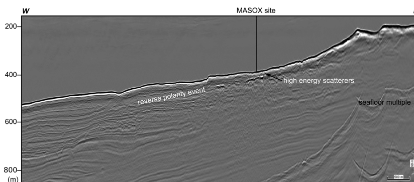
Figure 3. Prestack depth migrated line JR211-03 (after Sarkar et al., 2012) showing reverse polarity at shallow depth indicating the presence of free gas. The MASOX site is at the transition from glaciogenic diamictites in the east to a contouritic glaciomarine sedimentation in the west.
