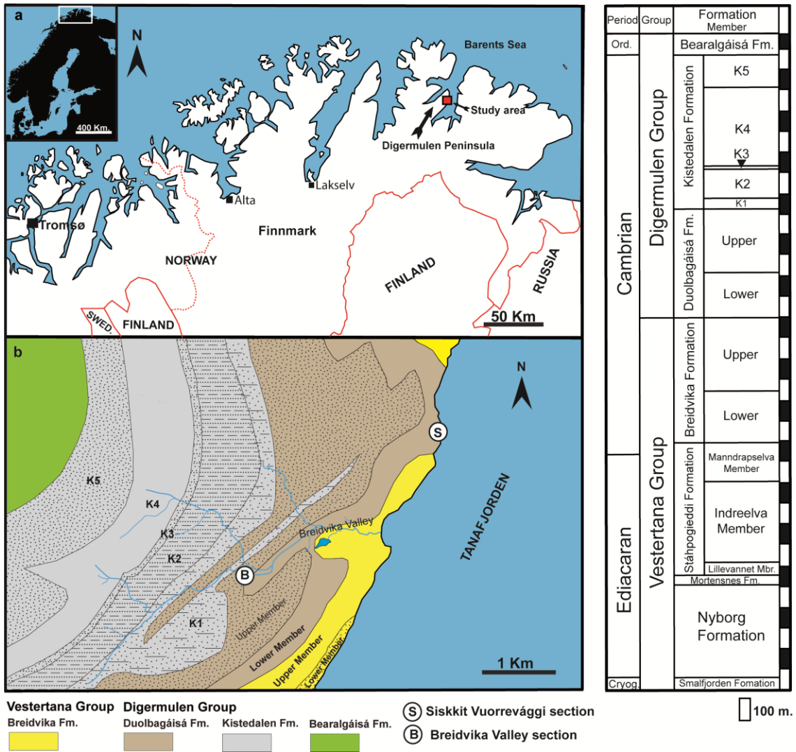
Fig. 1. Location and geological setting of study area on the Digermulen Peninsula, Arctic Norway. (a) Geographical location of the Digermulen Peninsula. (b) Geology of the Breidvika Valley area with location of the Duolbagáisá Formation sections of this study.
