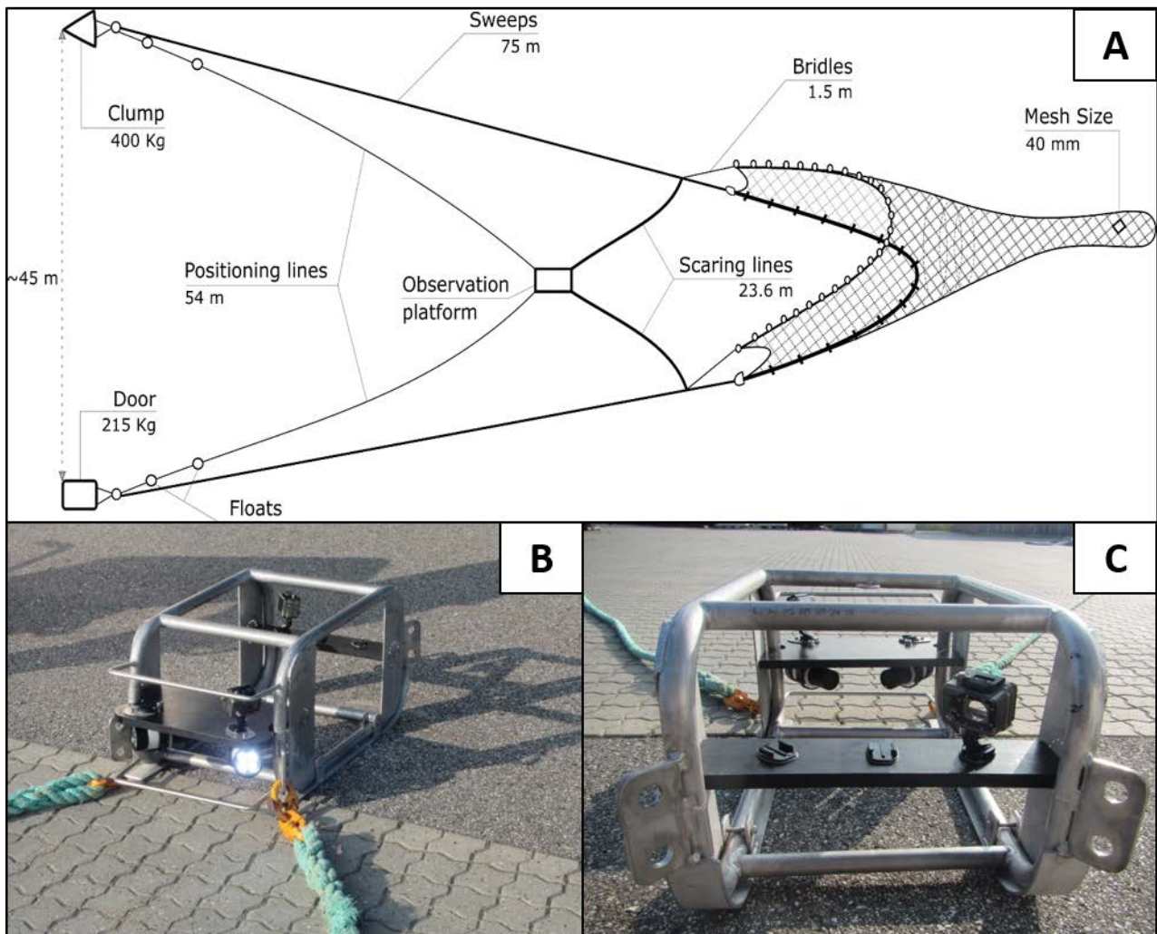
129 130 Figure 1. A) The port side trawl in a twin-rig system with FLEXSELECT raised (adapted from Melli et al. 2018). 131 Proportions are not respected to facilitate the identification of all components; B) observation platform (back 132 view) with scaring lines; C) observation platform (front view). During the experimental trials floats were 133 attached to the top of the observation platform.
