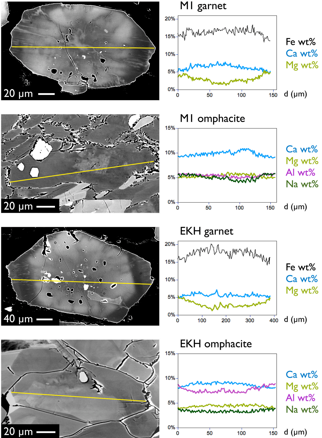
Fig. 5. Element concentration profiles for garnet and omphacite. Concentrations along profiles across garnet and omphacite grains from the Bohemian massif (M1) and the Tauern Window (EKH) eclogites are shown.
