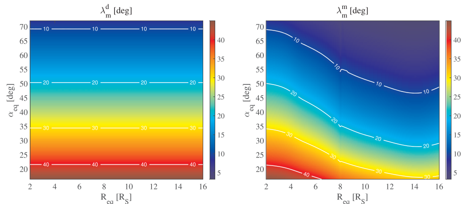
Figure 6. Same figure as Figure 2 with latitude for mirror point but for the Kronian system.
