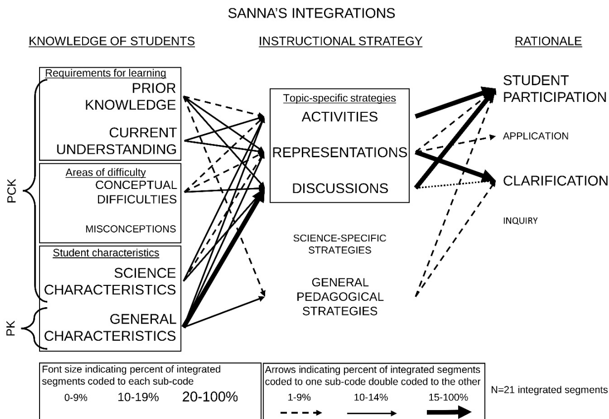
Figure 2. All integrated segment coding for Sanna, represented in a PCK map
