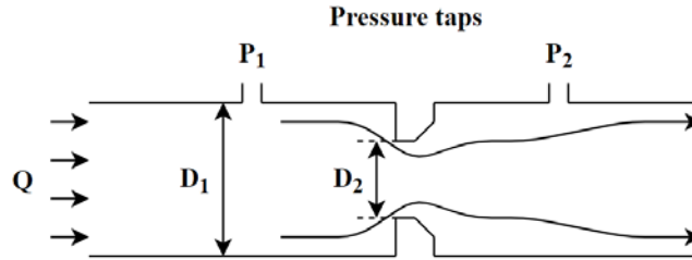
Figure 1 - Orifice plate arrangement in a pipeline
