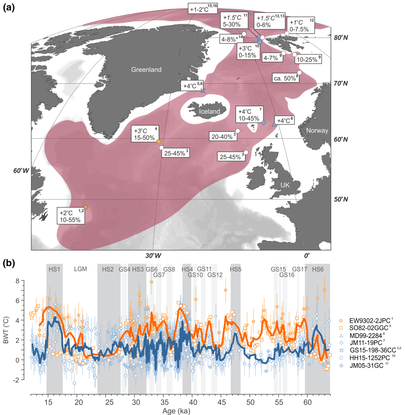
Figure 6. (a) Compilation of core records from the northern North Atlantic Ocean, Nordic Seas, and Arctic Ocean containing the “Atlantic species” group (in percentage; sensu Rasmussen et al. (1996a), except for core no. 13, where the Atlantic species group follows the definition of Wollenburg et al. [2004]) and absolute bottom water temperatures (BWT) (°C) increases during Heinrich Stadials and Greenland Stadials. BWT increases were calculated as difference to the previous interstadial period. BWT given in italics were obtained from benthic foraminiferal transfer functions. Colored area indicates northward Atlantic subsurface intermediate water flow. (b) BWT records compilation for the last 64 ka for water depths between 800 and 1,500 m. Smoothed lines were obtained with five point weighted average. Symbols (orange for the North Atlantic and blue for the Nordic Seas) are the same as in panel (a) to identify each specific core location. References: 1 = Marcott et al. (2011); 2 = T. L. Rasmussen et al. (2003); 3 = T. L. Rasmussen & Thomsen (2004); 4 = T. L. Rasmussen & Thomsen (2017); 5 = Sessford et al. (2018); 6 = Sessford et al. (2019); 7 = Ezat et al. (2014); 8 = Danielsen (2017); 9 = T. L. Rasmussen et al. (2007); 10 = This work; 11 = T. L. Rasmussen et al. (2014b); 12 = Chauhan et al. (2016); 13 = Chauhan et al. (2014); 14 = Wollenburg et al. (2004); 15 = Cronin et al. (2012); 16 = Cronin et al. (2017).
